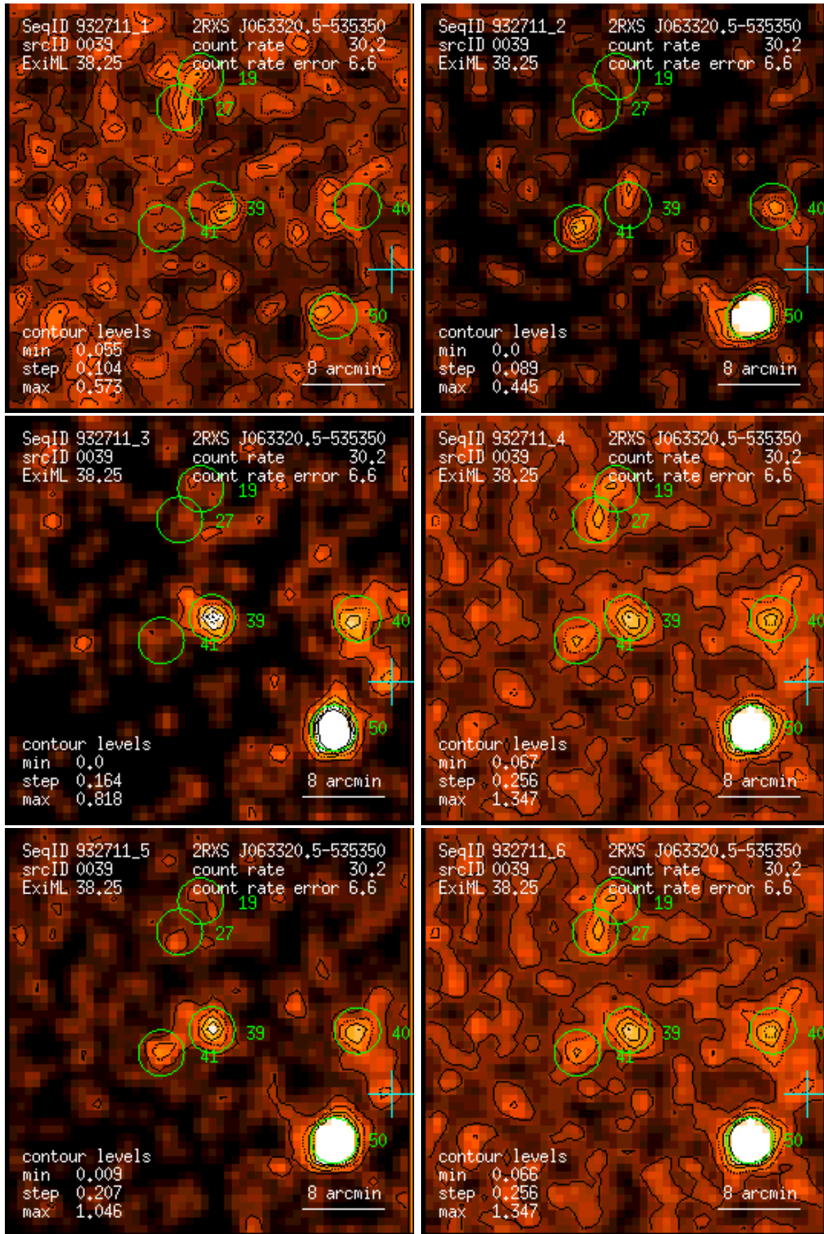
Figure 39: RASS 932711: detection 0039: band rate images, Gaussian filter: (1) PSPC channels 11 – 41, (2) 52 – 90, (3) 91 – 201, (4) 11 – 235, (5) 52 – 201, (6) 11 – 201. Broad band rates in counts/ks. Band rate contour levels in counts/ks/arcmin 2 .
