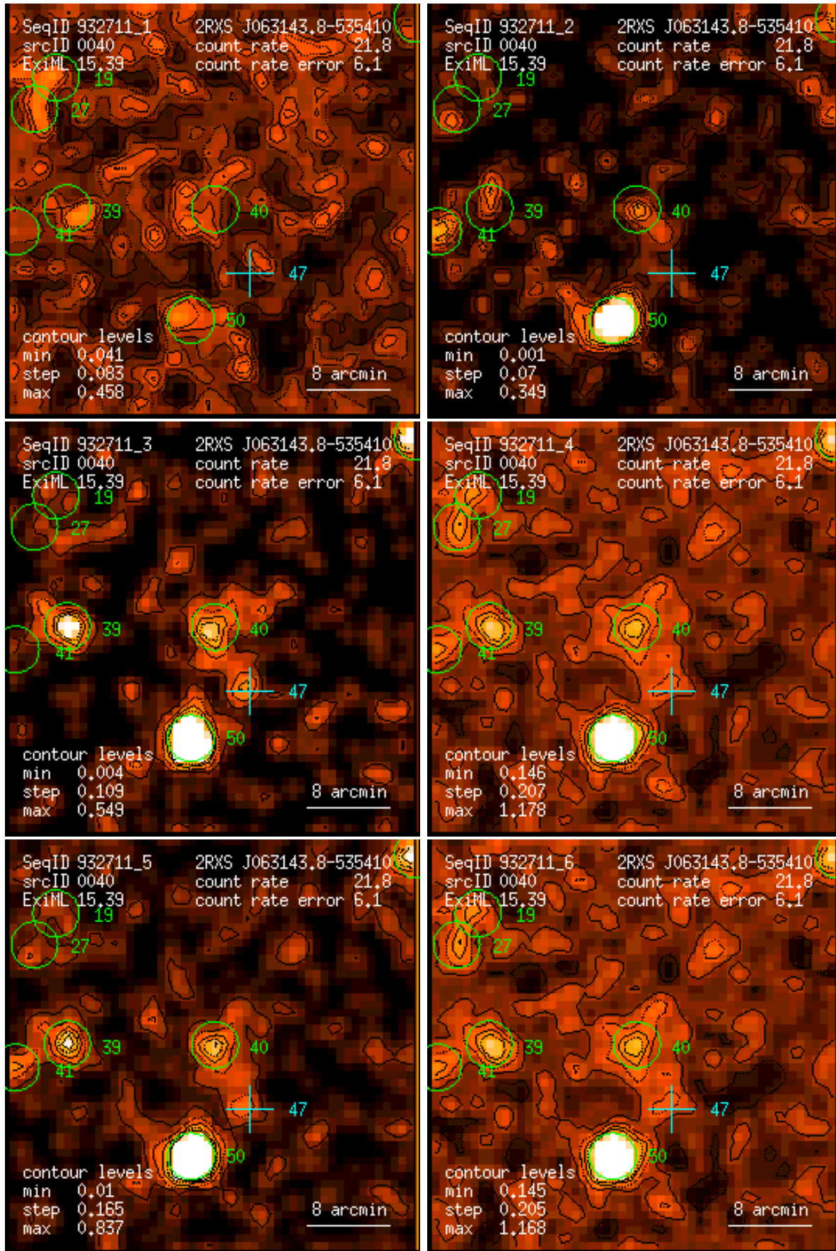
Figure 40: RASS 932711: detection 0040: band rate images, Gaussian filter: (1) PSPC channels 11 – 41, (2) 52 – 90, (3) 91 – 201, (4) 11 – 235, (5) 52 – 201, (6) 11 – 201. Broad band rates in counts/ks. Band rate contour levels in counts/ks/arcmin 2 .
