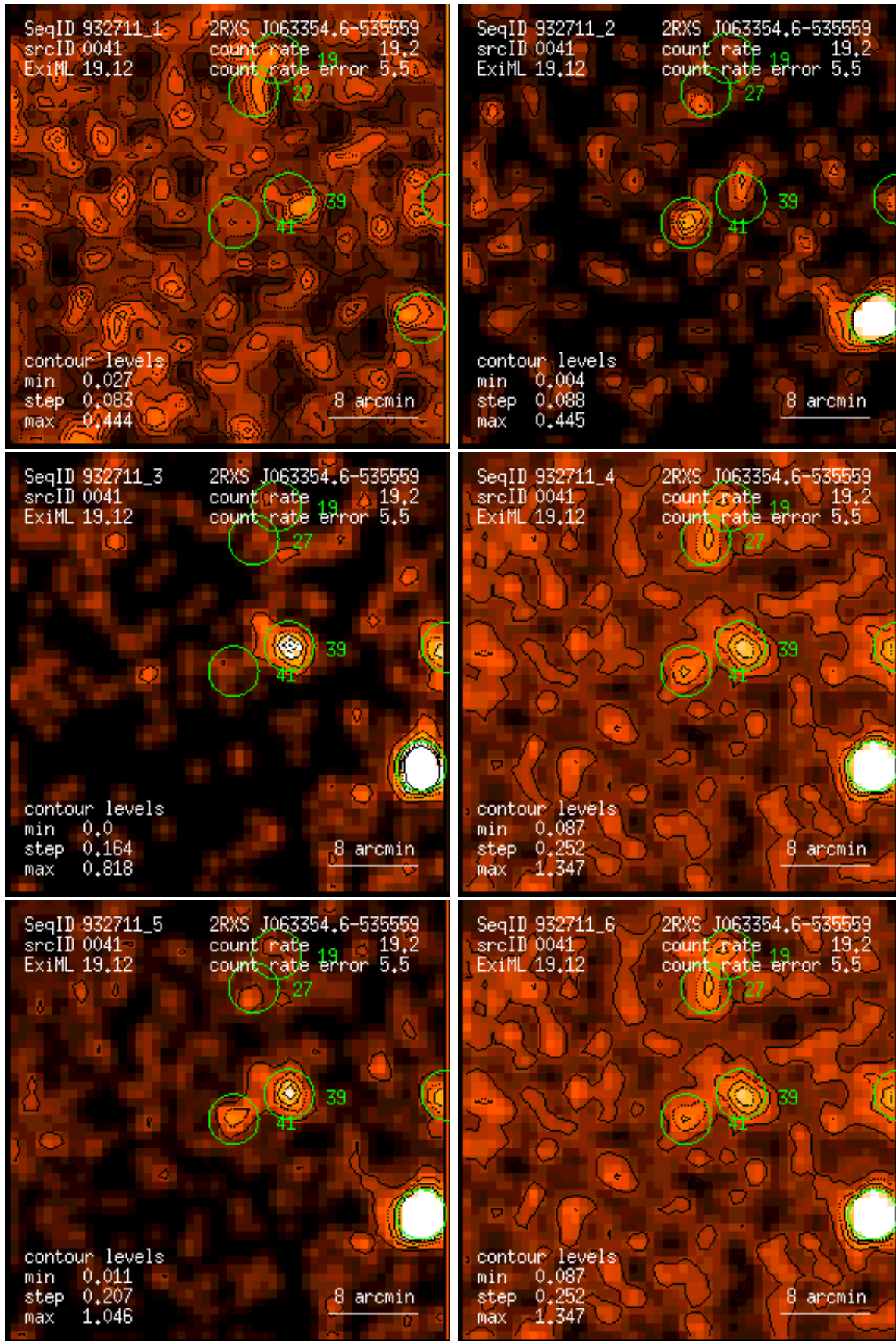
Figure 41: RASS 932711: detection 0041: band rate images, Gaussian filter: (1) PSPC channels 11 – 41, (2) 52 – 90, (3) 91 – 201, (4) 11 – 235, (5) 52 – 201, (6) 11 – 201. Broad band rates in counts/ks. Band rate contour levels in counts/ks/arcmin 2 .
