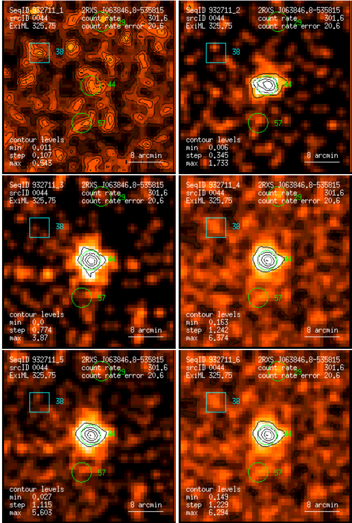
Figure 44: RASS 932711: detection 0044: band rate images, Gaussian filter: (1) PSPC channels 11 – 41, (2) 52 – 90, (3) 91 – 201, (4) 11 – 235, (5) 52 – 201, (6) 11 – 201. Broad band rates in counts/ks. Band rate contour levels in counts/ks/arcmin 2 .
