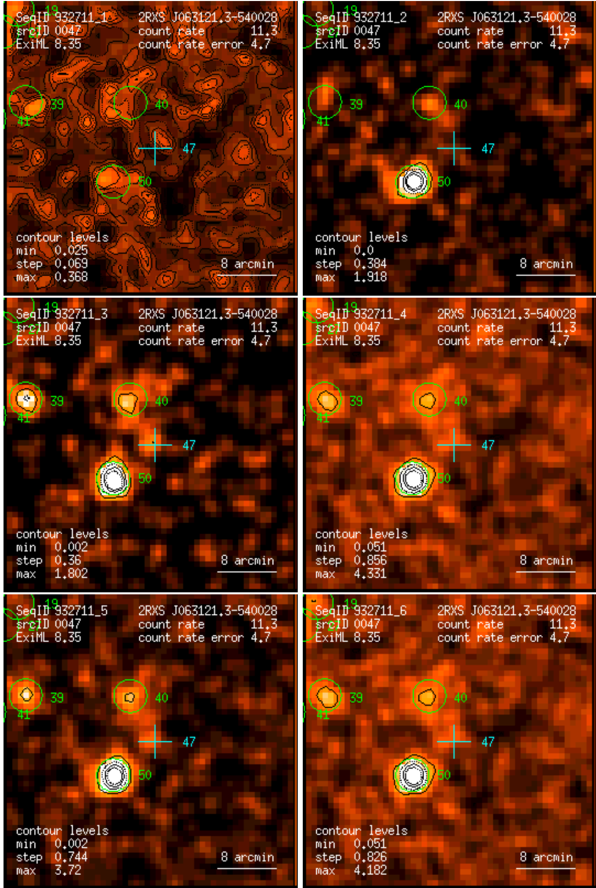
Figure 47: RASS 932711: detection 0047: band rate images, Gaussian filter: (1) PSPC channels 11 – 41, (2) 52 – 90, (3) 91 – 201, (4) 11 – 235, (5) 52 – 201, (6) 11 – 201. Broad band rates in counts/ks. Band rate contour levels in counts/ks/arcmin 2 .
