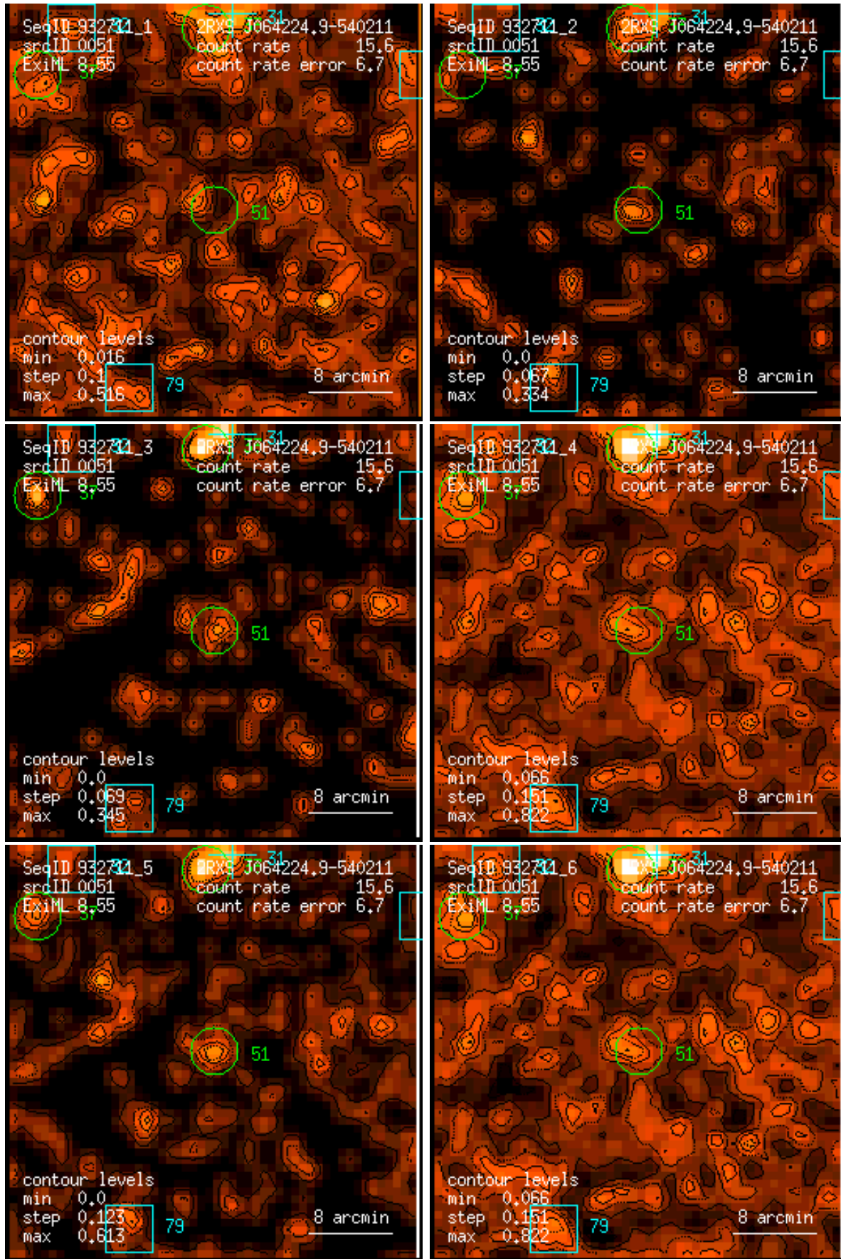
Figure 51: RASS 932711: detection 0051: band rate images, Gaussian filter: (1) PSPC channels 11 – 41, (2) 52 – 90, (3) 91 – 201, (4) 11 – 235, (5) 52 – 201, (6) 11 – 201. Broad band rates in counts/ks. Band rate contour levels in counts/ks/arcmin 2 .
