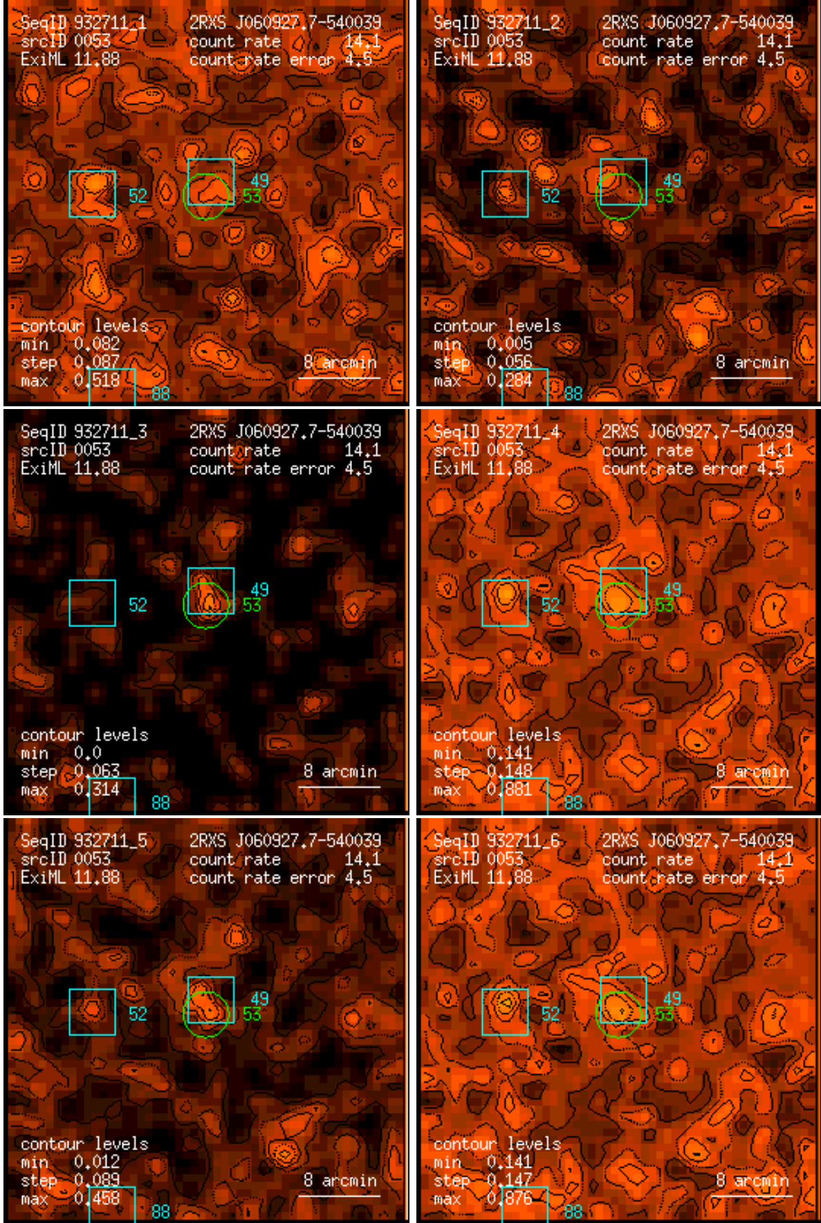
Figure 53: RASS 932711: detection 0053: band rate images, Gaussian filter: (1) PSPC channels 11 – 41, (2) 52 – 90, (3) 91 – 201, (4) 11 – 235, (5) 52 – 201, (6) 11 – 201. Broad band rates in counts/ks. Band rate contour levels in counts/ks/arcmin 2 .
