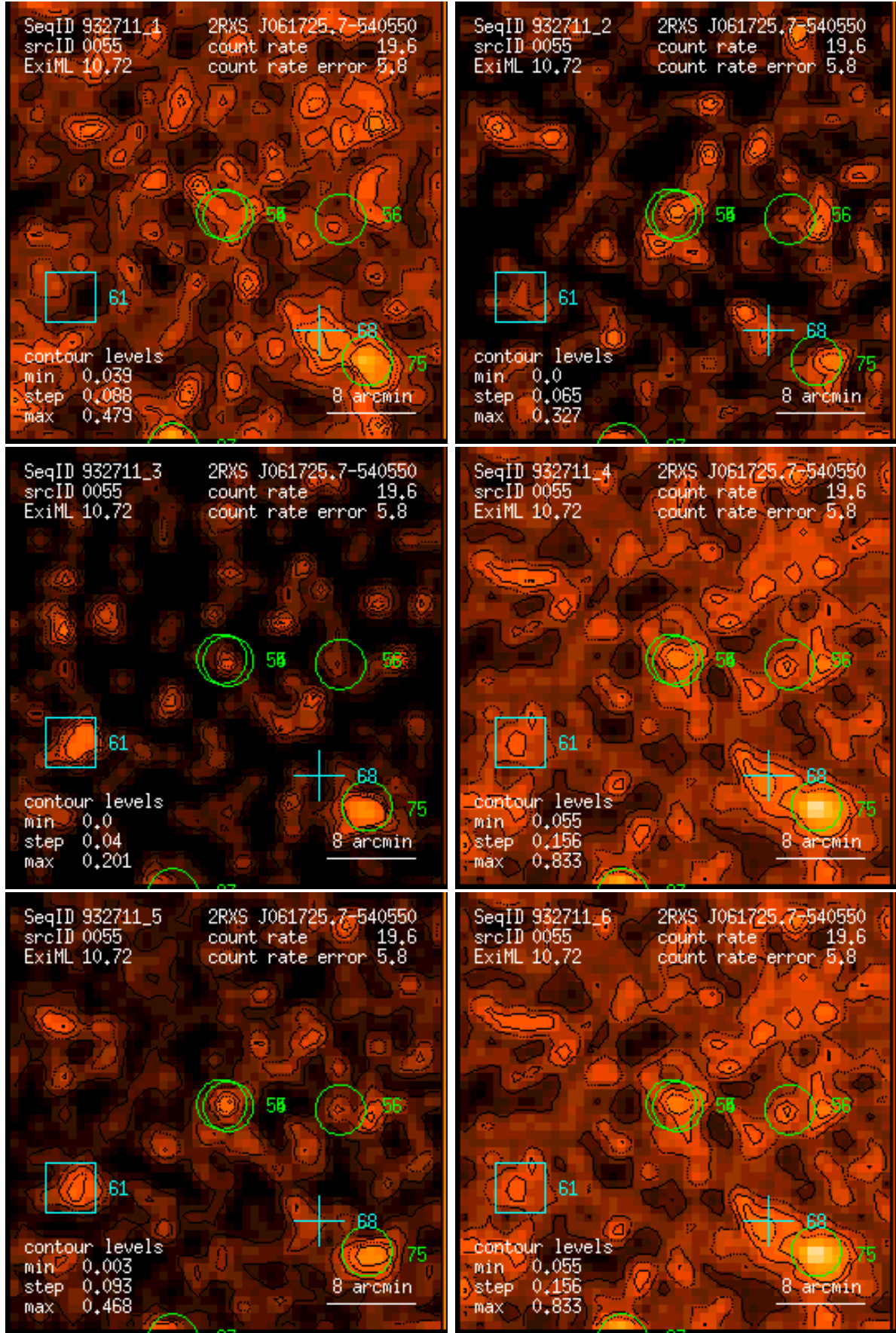
Figure 55: RASS 932711: detection 0055: band rate images, Gaussian filter: (1) PSPC channels 11 – 41, (2) 52 – 90, (3) 91 – 201, (4) 11 – 235, (5) 52 – 201, (6) 11 – 201. Broad band rates in counts/ks. Band rate contour levels in counts/ks/arcmin 2 .
