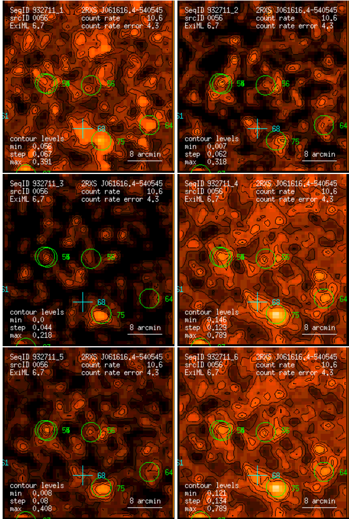
Figure 56: RASS 932711: detection 0056: band rate images, Gaussian filter: (1) PSPC channels 11 – 41, (2) 52 – 90, (3) 91 – 201, (4) 11 – 235, (5) 52 – 201, (6) 11 – 201. Broad band rates in counts/ks. Band rate contour levels in counts/ks/arcmin 2 .
