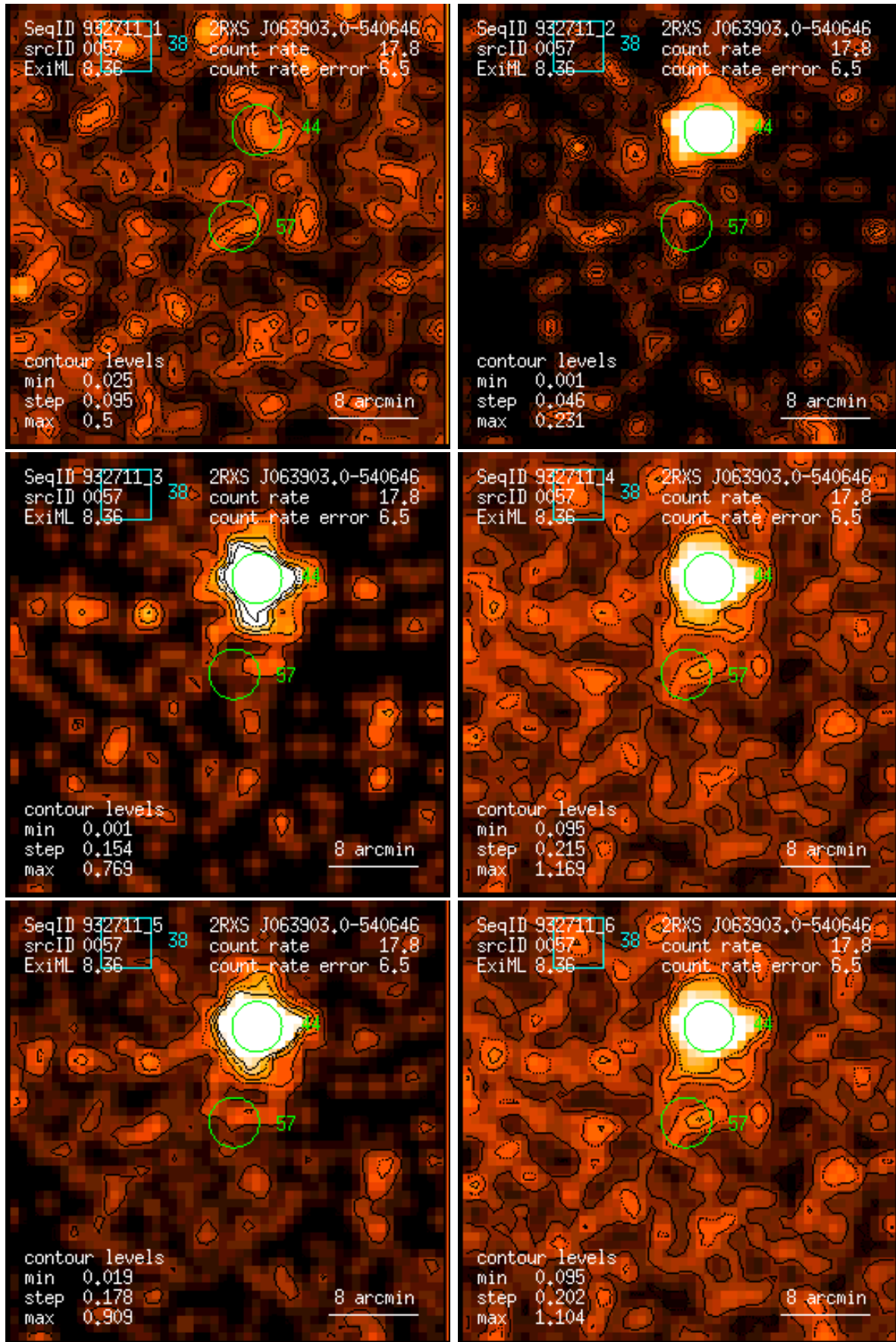
Figure 57: RASS 932711: detection 0057: band rate images, Gaussian filter: (1) PSPC channels 11 – 41, (2) 52 – 90, (3) 91 – 201, (4) 11 – 235, (5) 52 – 201, (6) 11 – 201. Broad band rates in counts/ks. Band rate contour levels in counts/ks/arcmin 2 .
