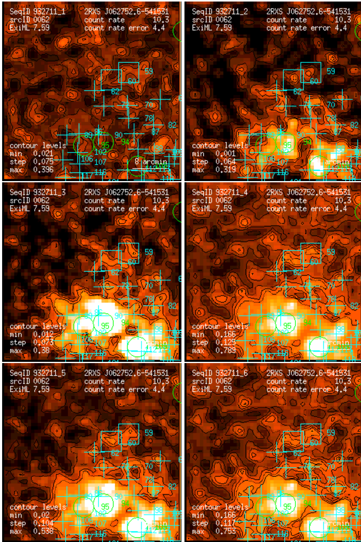
Figure 62: RASS 932711: detection 0062: band rate images, Gaussian filter: (1) PSPC channels 11 – 41, (2) 52 – 90, (3) 91 – 201, (4) 11 – 235, (5) 52 – 201, (6) 11 – 201. Broad band rates in counts/ks. Band rate contour levels in counts/ks/arcmin 2 .
