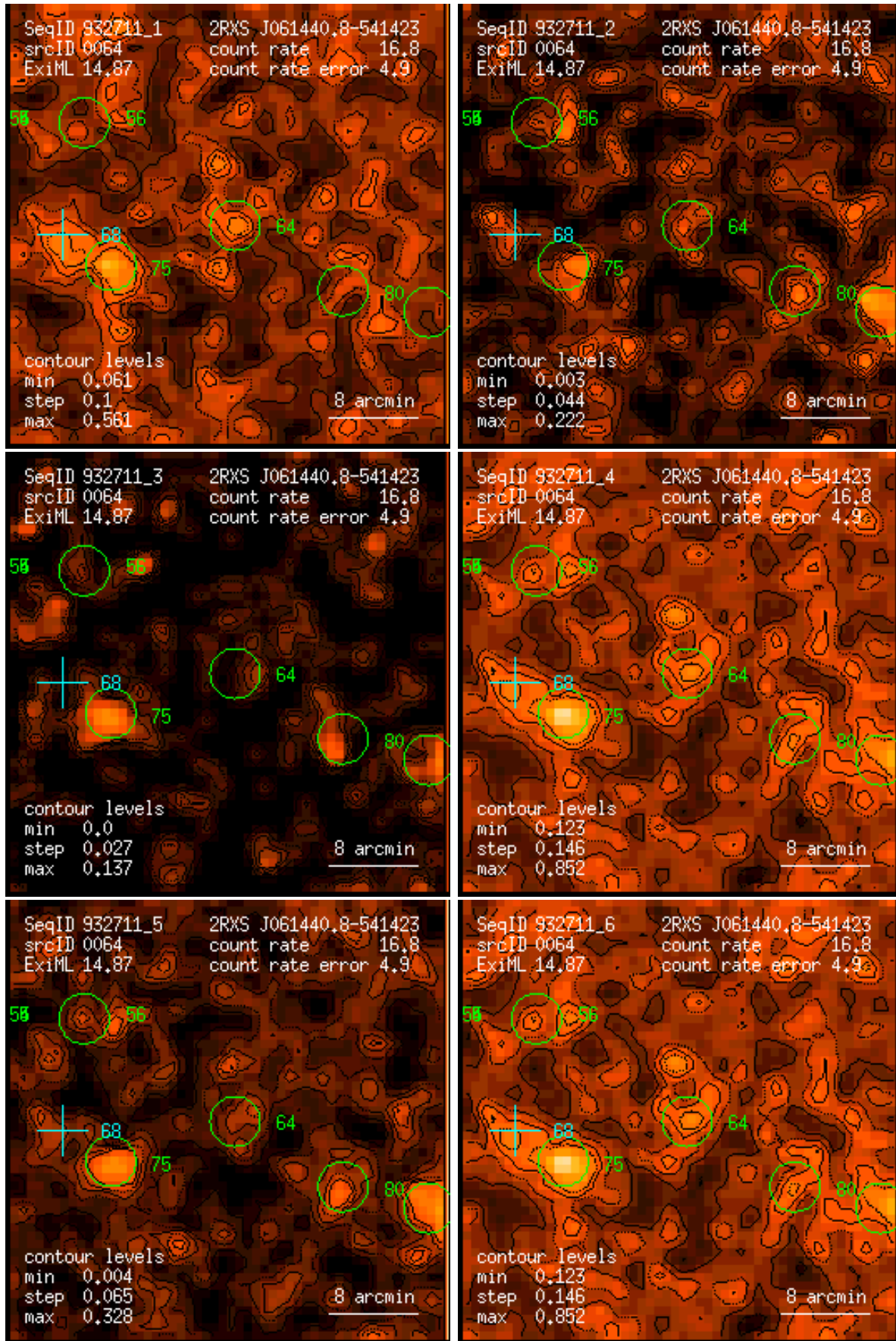
Figure 64: RASS 932711: detection 0064: band rate images, Gaussian filter: (1) PSPC channels 11 – 41, (2) 52 – 90, (3) 91 – 201, (4) 11 – 235, (5) 52 – 201, (6) 11 – 201. Broad band rates in counts/ks. Band rate contour levels in counts/ks/arcmin 2 .
