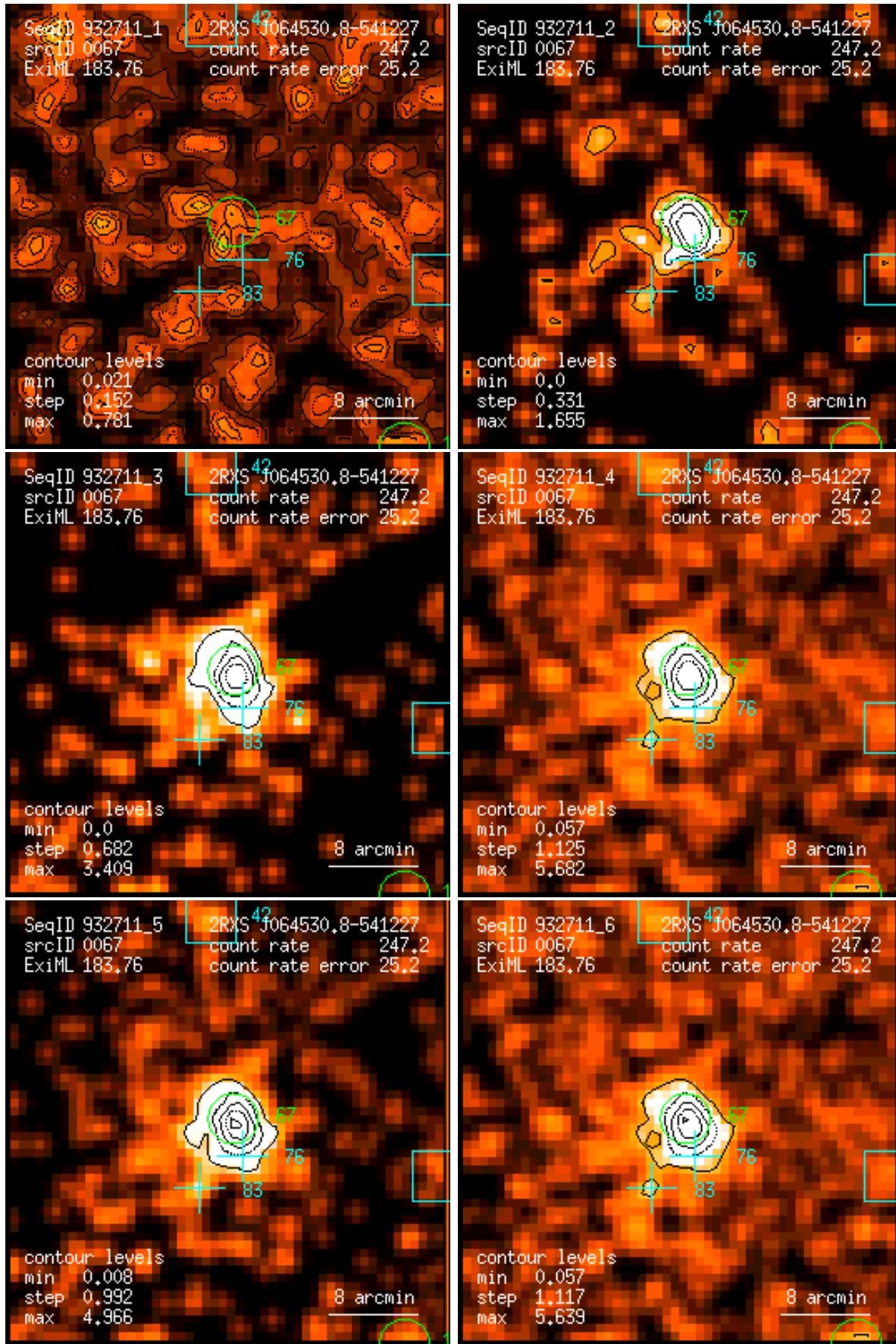
Figure 67: RASS 932711: detection 0067: band rate images, Gaussian filter: (1) PSPC channels 11 – 41, (2) 52 – 90, (3) 91 – 201, (4) 11 – 235, (5) 52 – 201, (6) 11 – 201. Broad band rates in counts/ks. Band rate contour levels in counts/ks/arcmin 2 .
