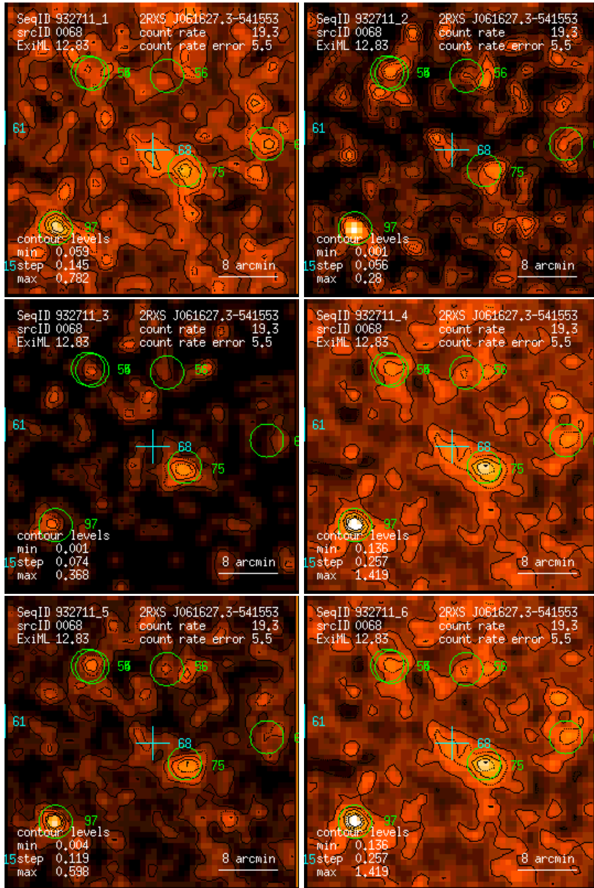
Figure 68: RASS 932711: detection 0068: band rate images, Gaussian filter: (1) PSPC channels 11 – 41, (2) 52 – 90, (3) 91 – 201, (4) 11 – 235, (5) 52 – 201, (6) 11 – 201. Broad band rates in counts/ks. Band rate contour levels in counts/ks/arcmin 2 .
