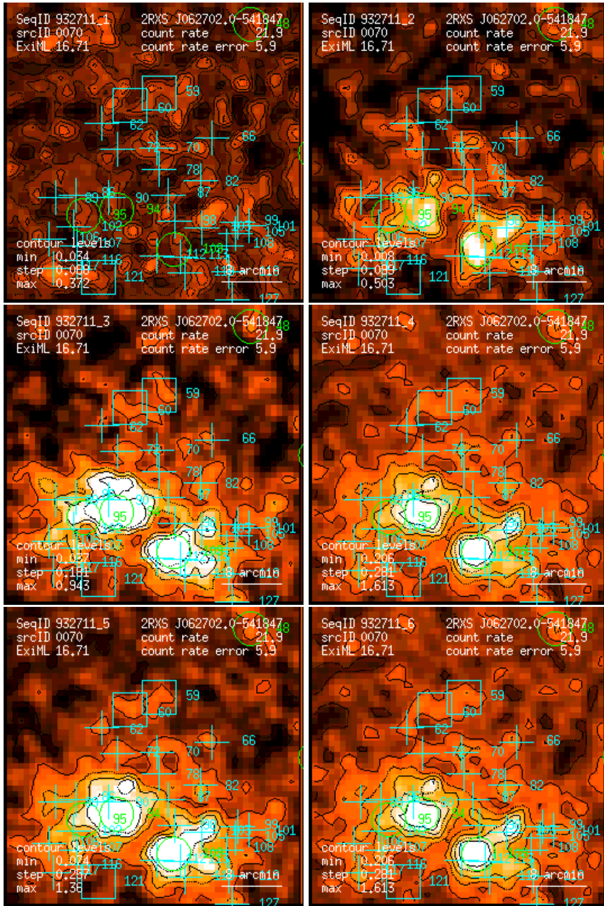
Figure 70: RASS 932711: detection 0070: band rate images, Gaussian filter: (1) PSPC channels 11 – 41, (2) 52 – 90, (3) 91 – 201, (4) 11 – 235, (5) 52 – 201, (6) 11 – 201. Broad band rates in counts/ks. Band rate contour levels in counts/ks/arcmin 2 .
