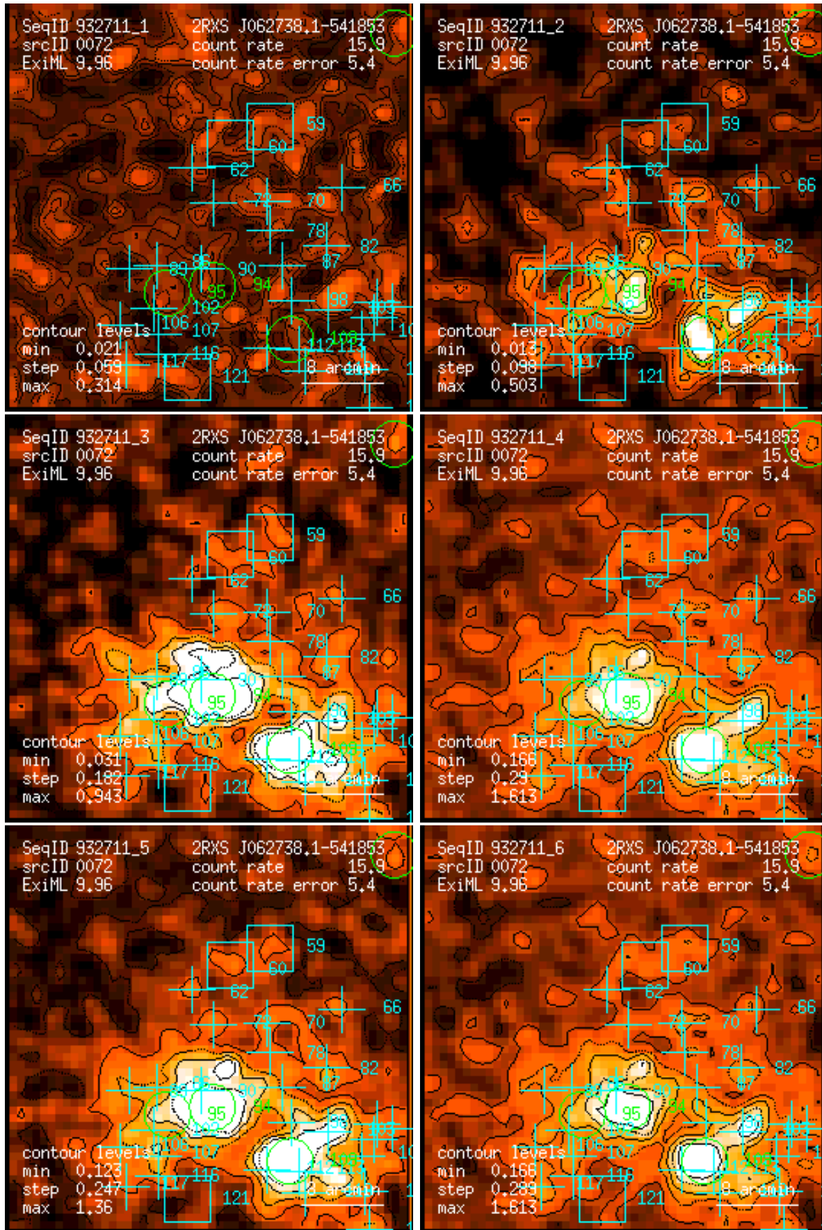
Figure 72: RASS 932711: detection 0072: band rate images, Gaussian filter: (1) PSPC channels 11 – 41, (2) 52 – 90, (3) 91 – 201, (4) 11 – 235, (5) 52 – 201, (6) 11 – 201. Broad band rates in counts/ks. Band rate contour levels in counts/ks/arcmin 2 .
