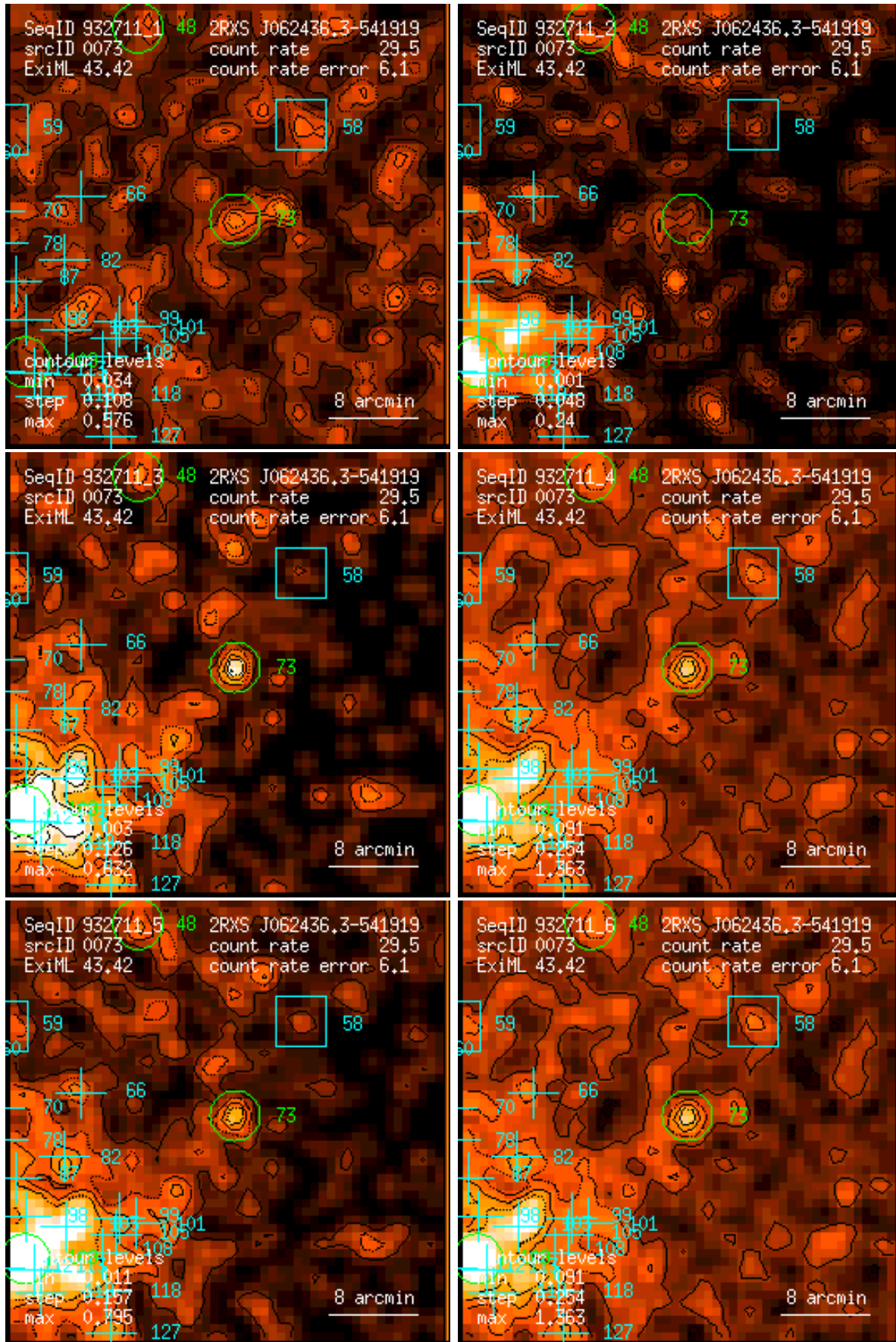
Figure 73: RASS 932711: detection 0073: band rate images, Gaussian filter: (1) PSPC channels 11 – 41, (2) 52 – 90, (3) 91 – 201, (4) 11 – 235, (5) 52 – 201, (6) 11 – 201. Broad band rates in counts/ks. Band rate contour levels in counts/ks/arcmin 2 .
