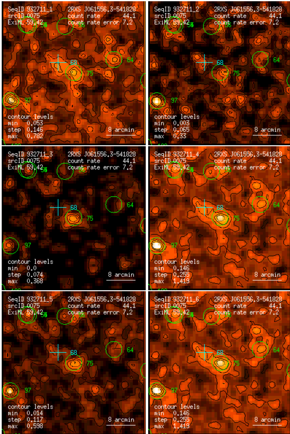
Figure 75: RASS 932711: detection 0075: band rate images, Gaussian filter: (1) PSPC channels 11 – 41, (2) 52 – 90, (3) 91 – 201, (4) 11 – 235, (5) 52 – 201, (6) 11 – 201. Broad band rates in counts/ks. Band rate contour levels in counts/ks/arcmin 2 .
