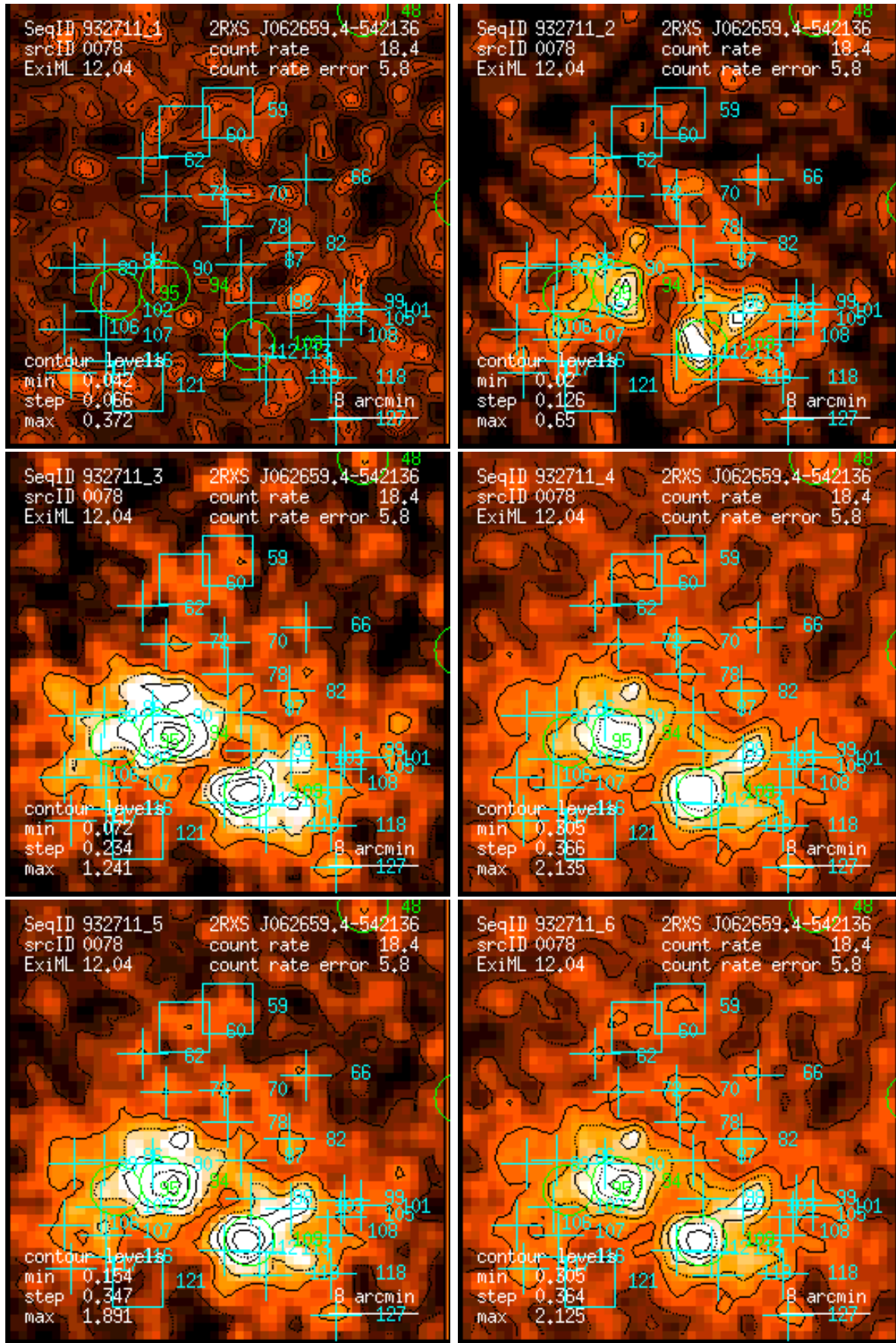
Figure 78: RASS 932711: detection 0078: band rate images, Gaussian filter: (1) PSPC channels 11 – 41, (2) 52 – 90, (3) 91 – 201, (4) 11 – 235, (5) 52 – 201, (6) 11 – 201. Broad band rates in counts/ks. Band rate contour levels in counts/ks/arcmin 2 .
