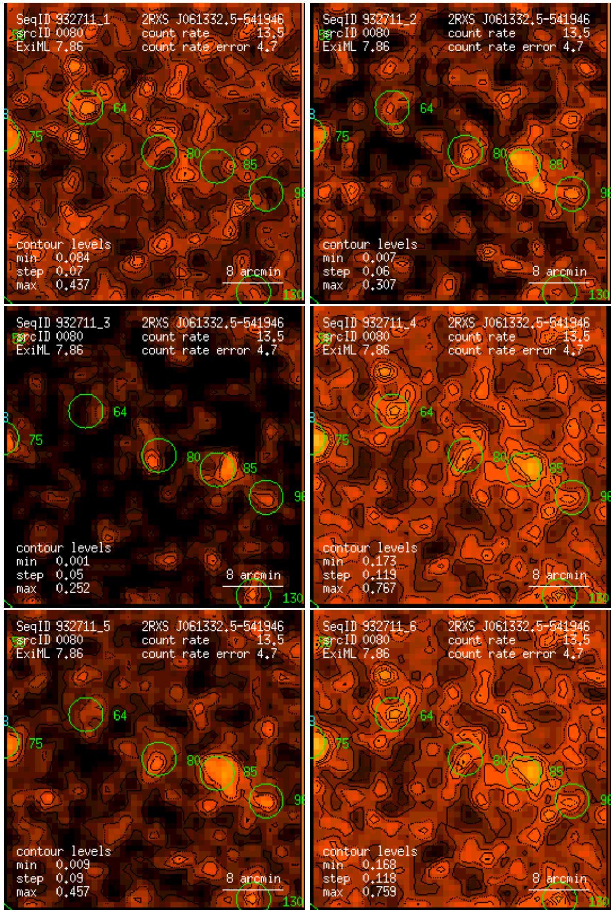
Figure 80: RASS 932711: detection 0080: band rate images, Gaussian filter: (1) PSPC channels 11 – 41, (2) 52 – 90, (3) 91 – 201, (4) 11 – 235, (5) 52 – 201, (6) 11 – 201. Broad band rates in counts/ks. Band rate contour levels in counts/ks/arcmin 2 .
