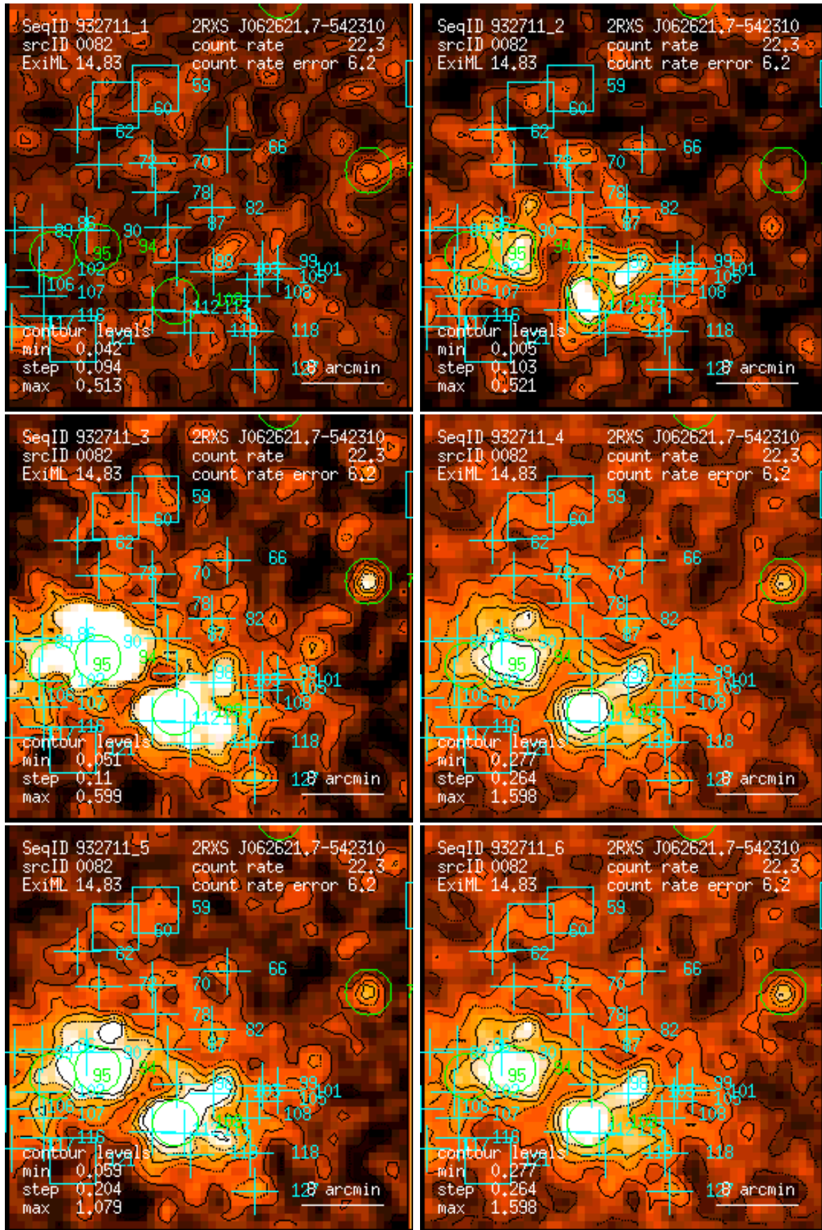
Figure 82: RASS 932711: detection 0082: band rate images, Gaussian filter: (1) PSPC channels 11 – 41, (2) 52 – 90, (3) 91 – 201, (4) 11 – 235, (5) 52 – 201, (6) 11 – 201. Broad band rates in counts/ks. Band rate contour levels in counts/ks/arcmin 2 .
