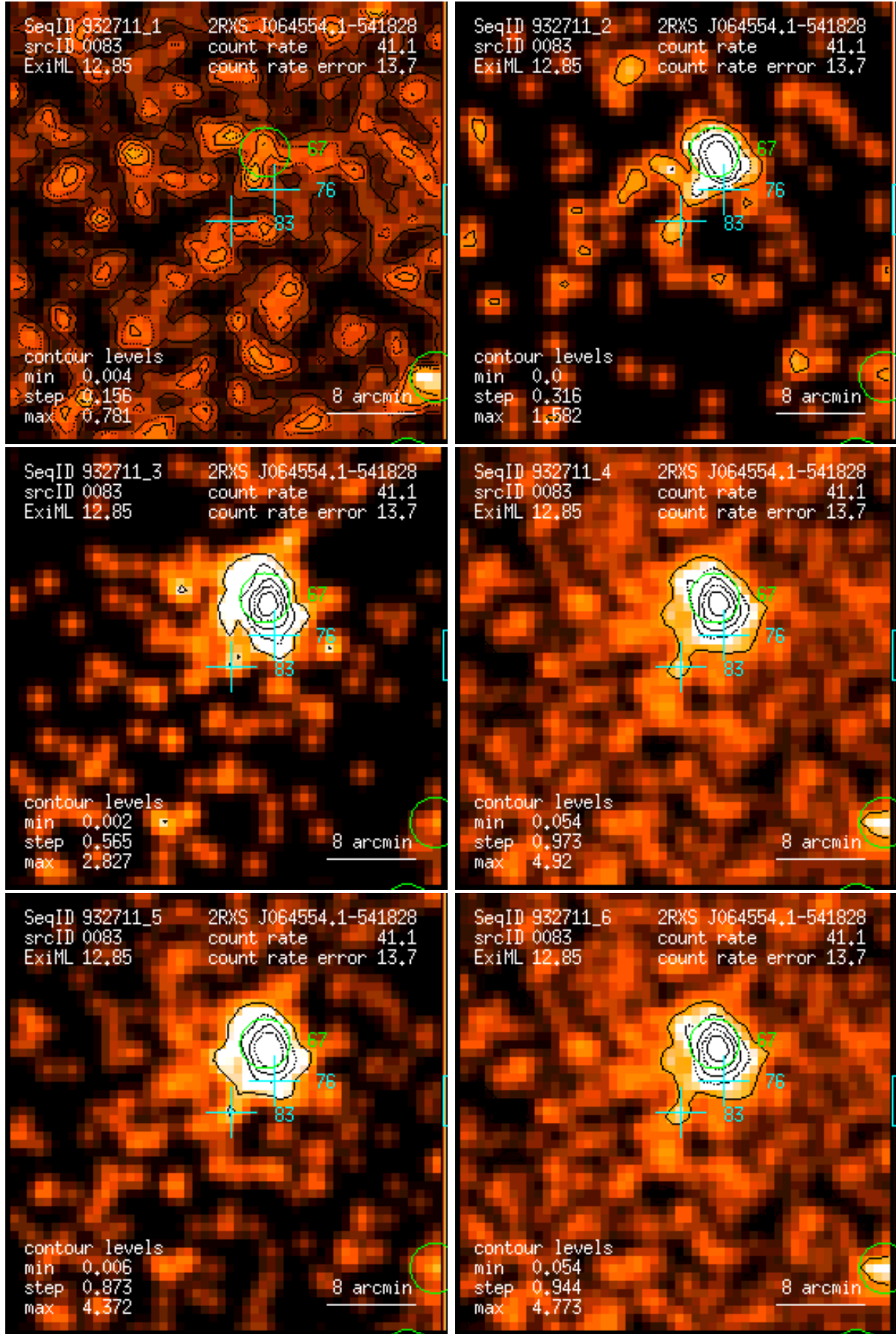
Figure 83: RASS 932711: detection 0083: band rate images, Gaussian filter: (1) PSPC channels 11 – 41, (2) 52 – 90, (3) 91 – 201, (4) 11 – 235, (5) 52 – 201, (6) 11 – 201. Broad band rates in counts/ks. Band rate contour levels in counts/ks/arcmin 2 .
