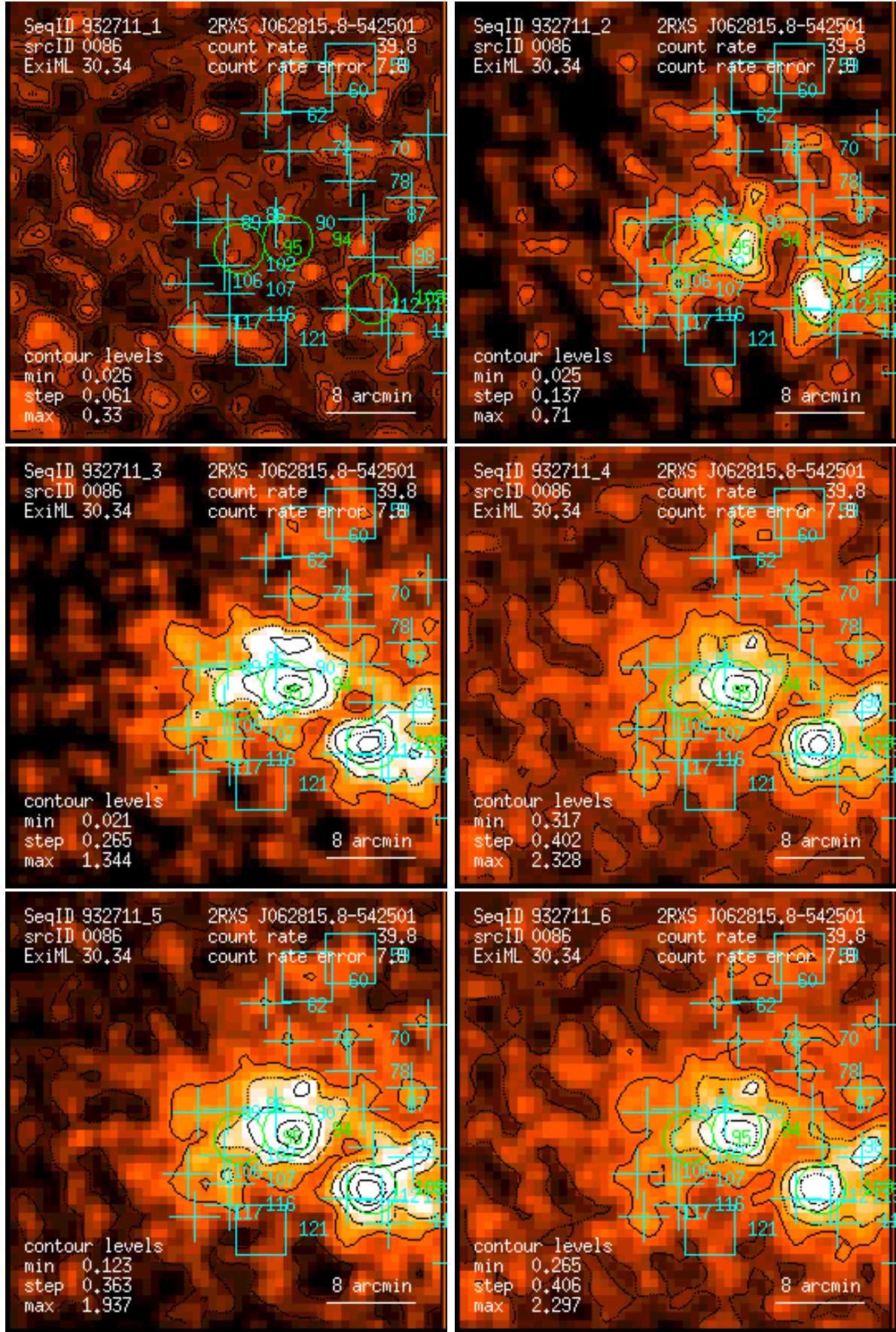
Figure 86: RASS 932711: detection 0086: band rate images, Gaussian filter: (1) PSPC channels 11 – 41, (2) 52 – 90, (3) 91 – 201, (4) 11 – 235, (5) 52 – 201, (6) 11 – 201. Broad band rates in counts/ks. Band rate contour levels in counts/ks/arcmin 2 .
