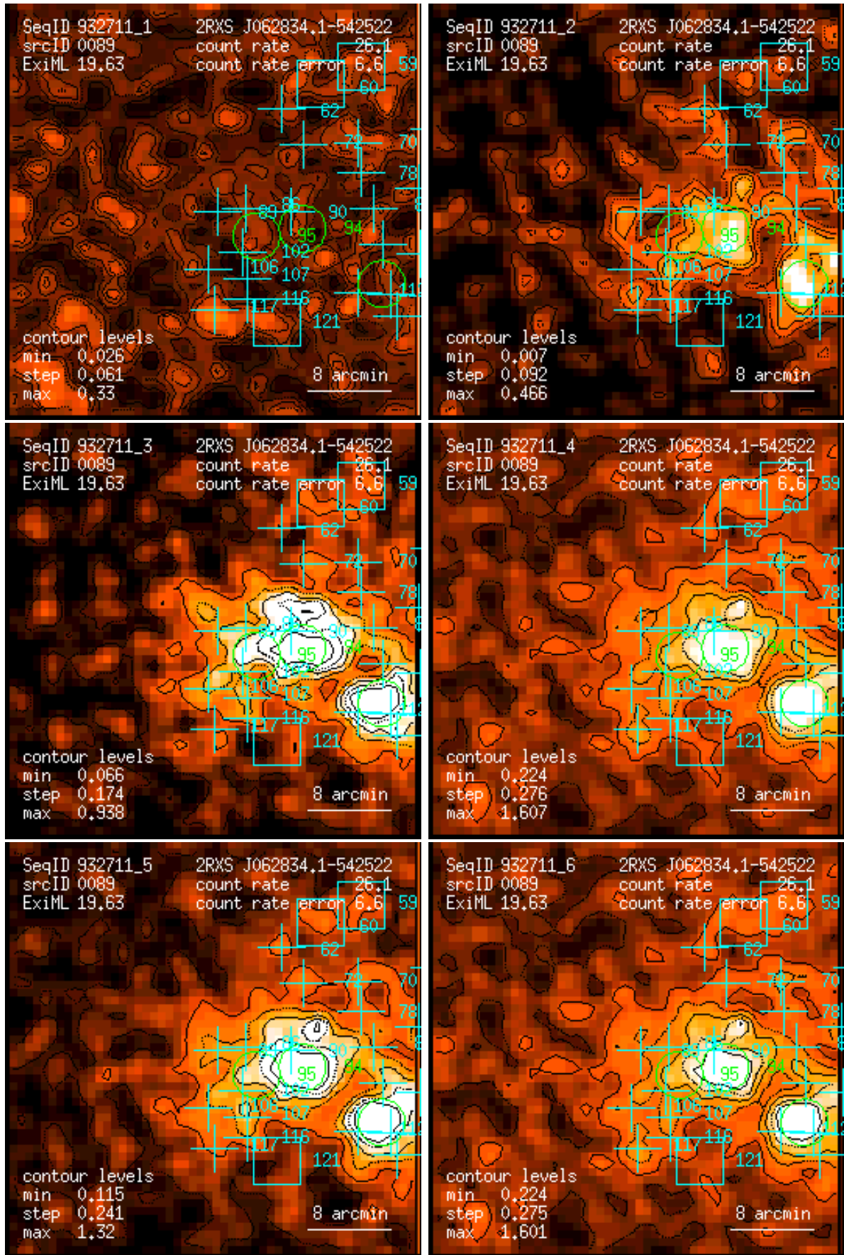
Figure 89: RASS 932711: detection 0089: band rate images, Gaussian filter: (1) PSPC channels 11 – 41, (2) 52 – 90, (3) 91 – 201, (4) 11 – 235, (5) 52 – 201, (6) 11 – 201. Broad band rates in counts/ks. Band rate contour levels in counts/ks/arcmin 2 .
