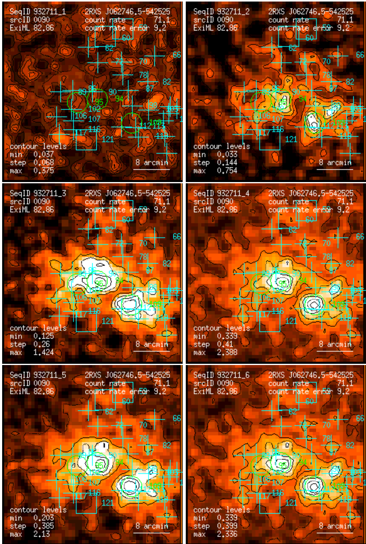
Figure 90: RASS 932711: detection 0090: band rate images, Gaussian filter: (1) PSPC channels 11 – 41, (2) 52 – 90, (3) 91 – 201, (4) 11 – 235, (5) 52 – 201, (6) 11 – 201. Broad band rates in counts/ks. Band rate contour levels in counts/ks/arcmin 2 .
