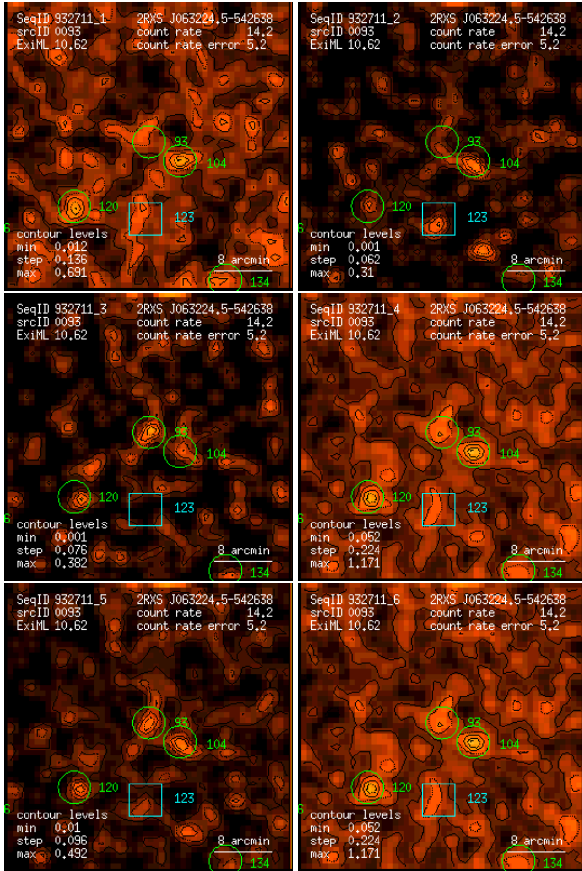
Figure 93: RASS 932711: detection 0093: band rate images, Gaussian filter: (1) PSPC channels 11 – 41, (2) 52 – 90, (3) 91 – 201, (4) 11 – 235, (5) 52 – 201, (6) 11 – 201. Broad band rates in counts/ks. Band rate contour levels in counts/ks/arcmin 2 .
