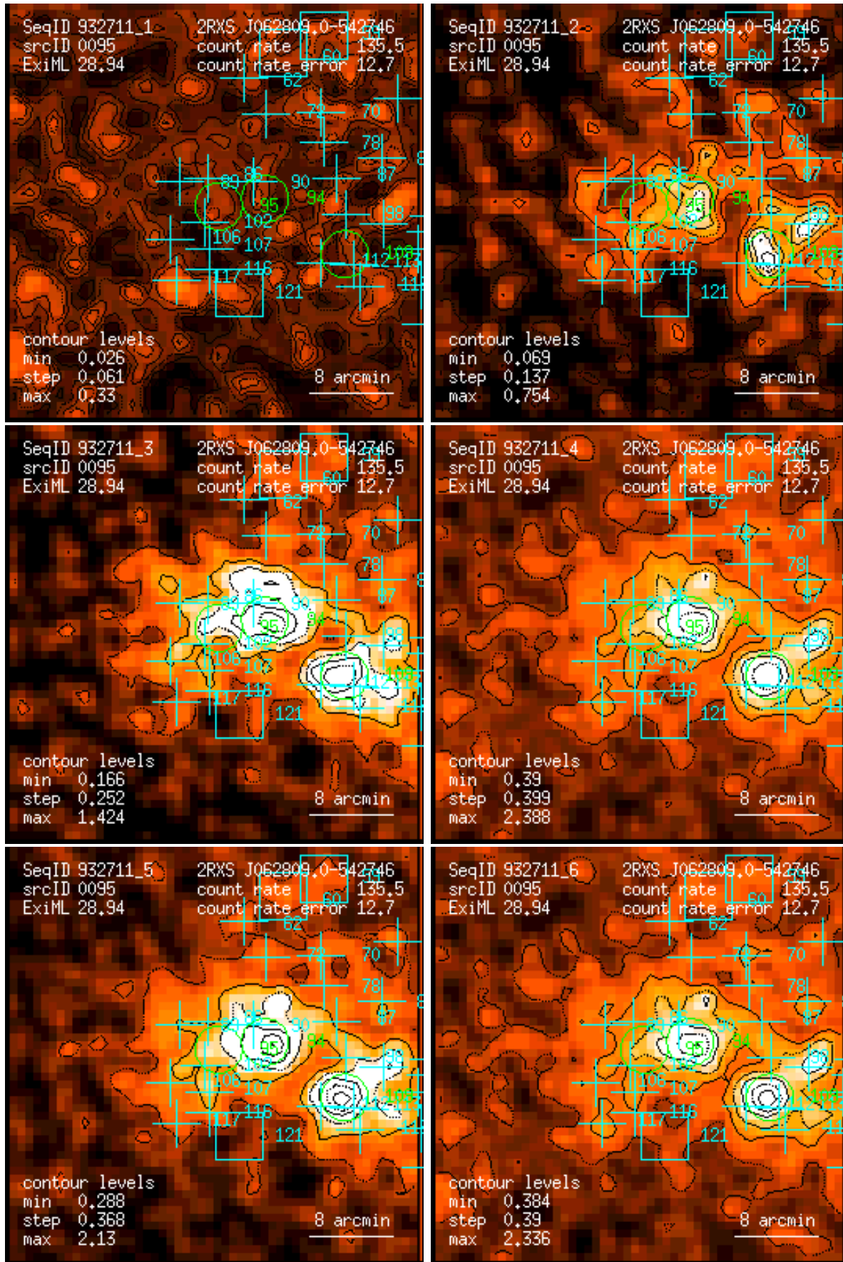
Figure 95: RASS 932711: detection 0095: band rate images, Gaussian filter: (1) PSPC channels 11 – 41, (2) 52 – 90, (3) 91 – 201, (4) 11 – 235, (5) 52 – 201, (6) 11 – 201. Broad band rates in counts/ks. Band rate contour levels in counts/ks/arcmin 2 .
