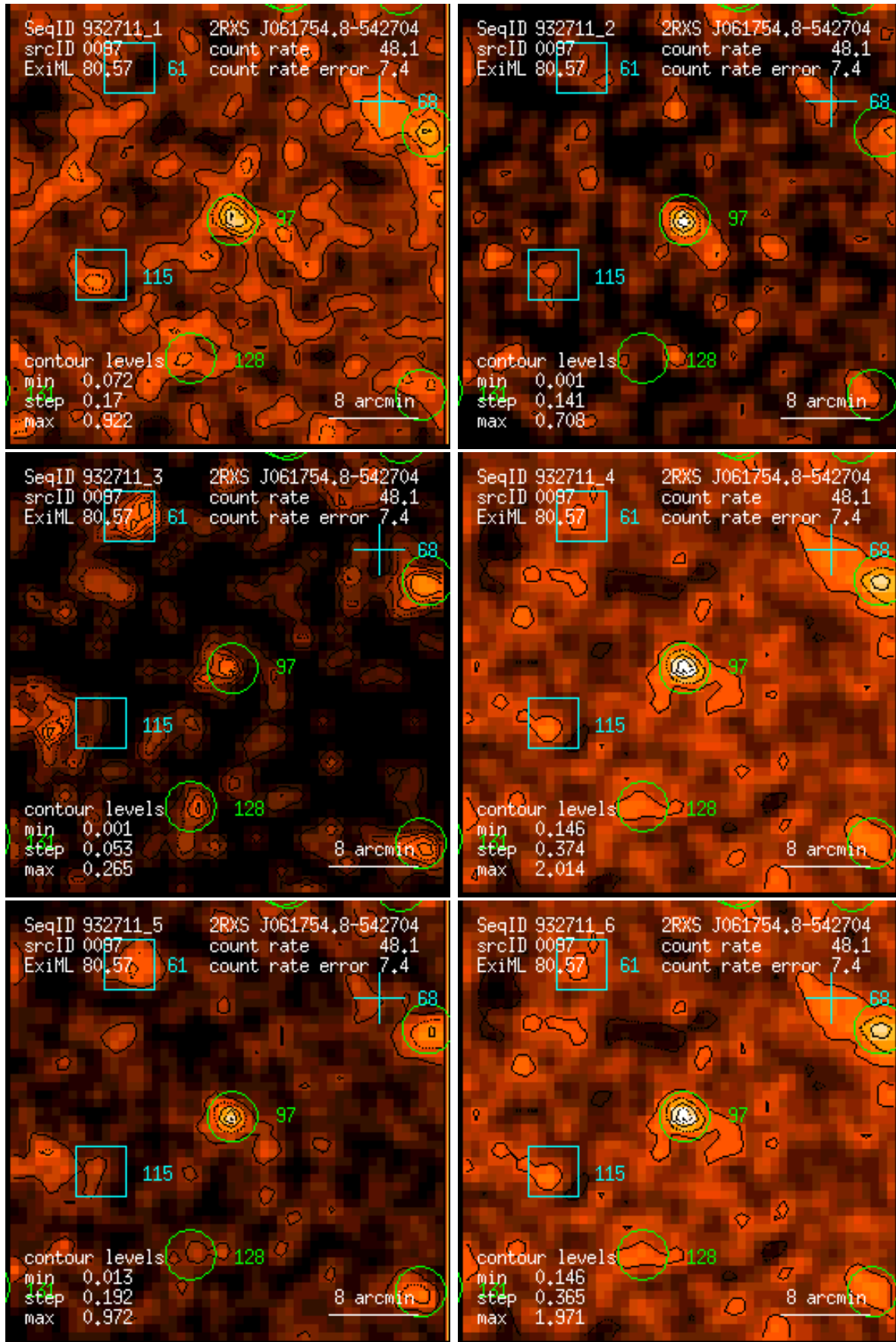
Figure 97: RASS 932711: detection 0097: band rate images, Gaussian filter: (1) PSPC channels 11 – 41, (2) 52 – 90, (3) 91 – 201, (4) 11 – 235, (5) 52 – 201, (6) 11 – 201. Broad band rates in counts/ks. Band rate contour levels in counts/ks/arcmin 2 .
