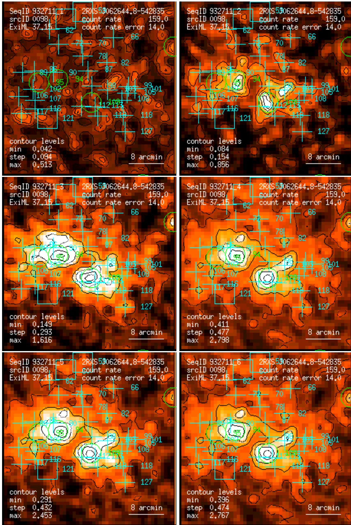
Figure 98: RASS 932711: detection 0098: band rate images, Gaussian filter: (1) PSPC channels 11 – 41, (2) 52 – 90, (3) 91 – 201, (4) 11 – 235, (5) 52 – 201, (6) 11 – 201. Broad band rates in counts/ks. Band rate contour levels in counts/ks/arcmin 2 .
