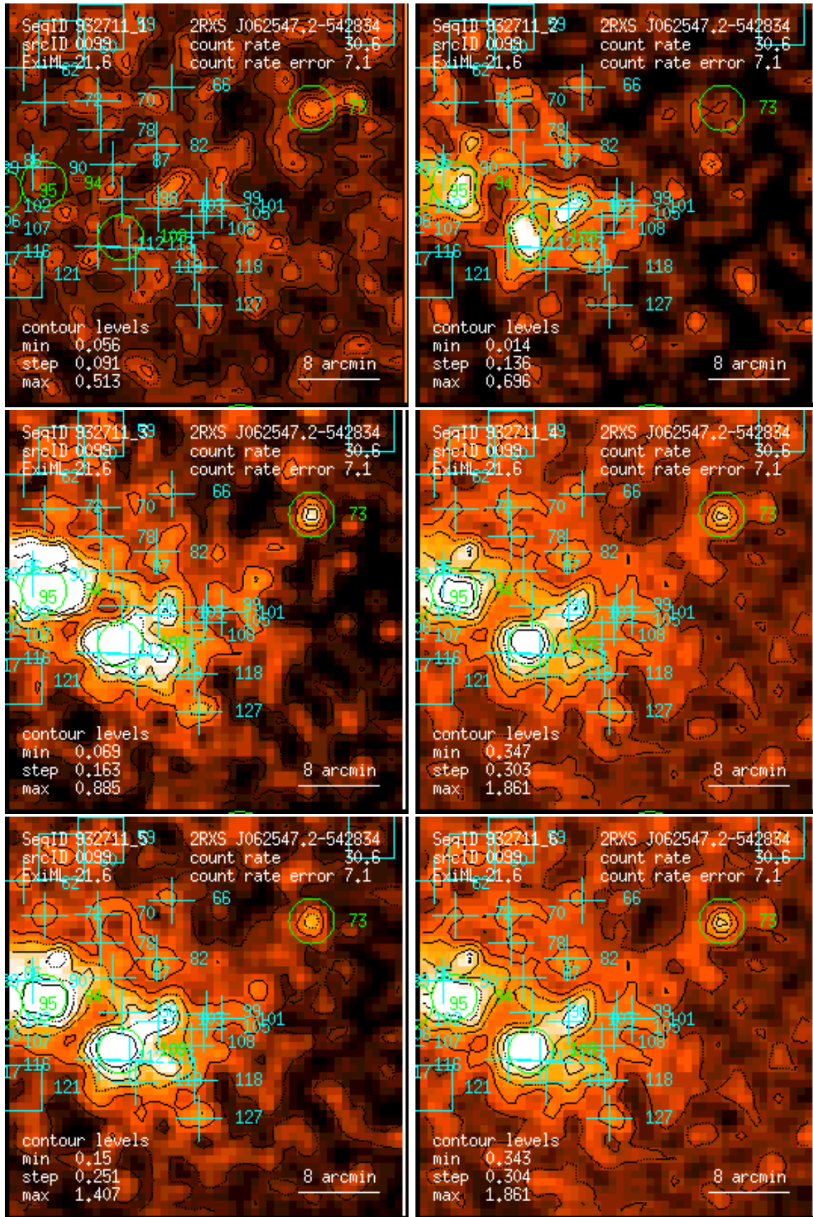
Figure 99: RASS 932711: detection 0099: band rate images, Gaussian filter: (1) PSPC channels 11 – 41, (2) 52 – 90, (3) 91 – 201, (4) 11 – 235, (5) 52 – 201, (6) 11 – 201. Broad band rates in counts/ks. Band rate contour levels in counts/ks/arcmin 2 .
