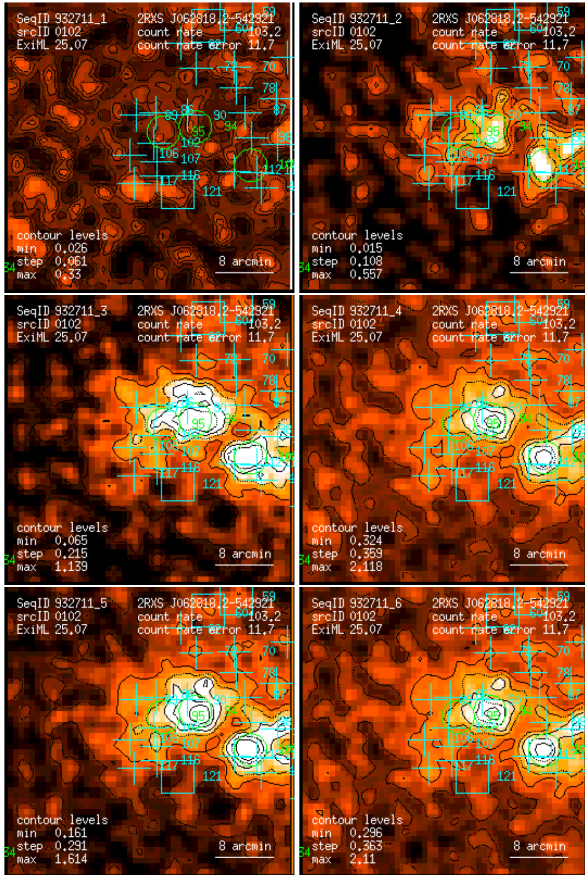
Figure 102: RASS 932711: detection 0102: band rate images, Gaussian filter: (1) PSPC channels 11 – 41, (2) 52 – 90, (3) 91 – 201, (4) 11 – 235, (5) 52 – 201, (6) 11 – 201. Broad band rates in counts/ks. Band rate contour levels in counts/ks/arcmin 2 .
