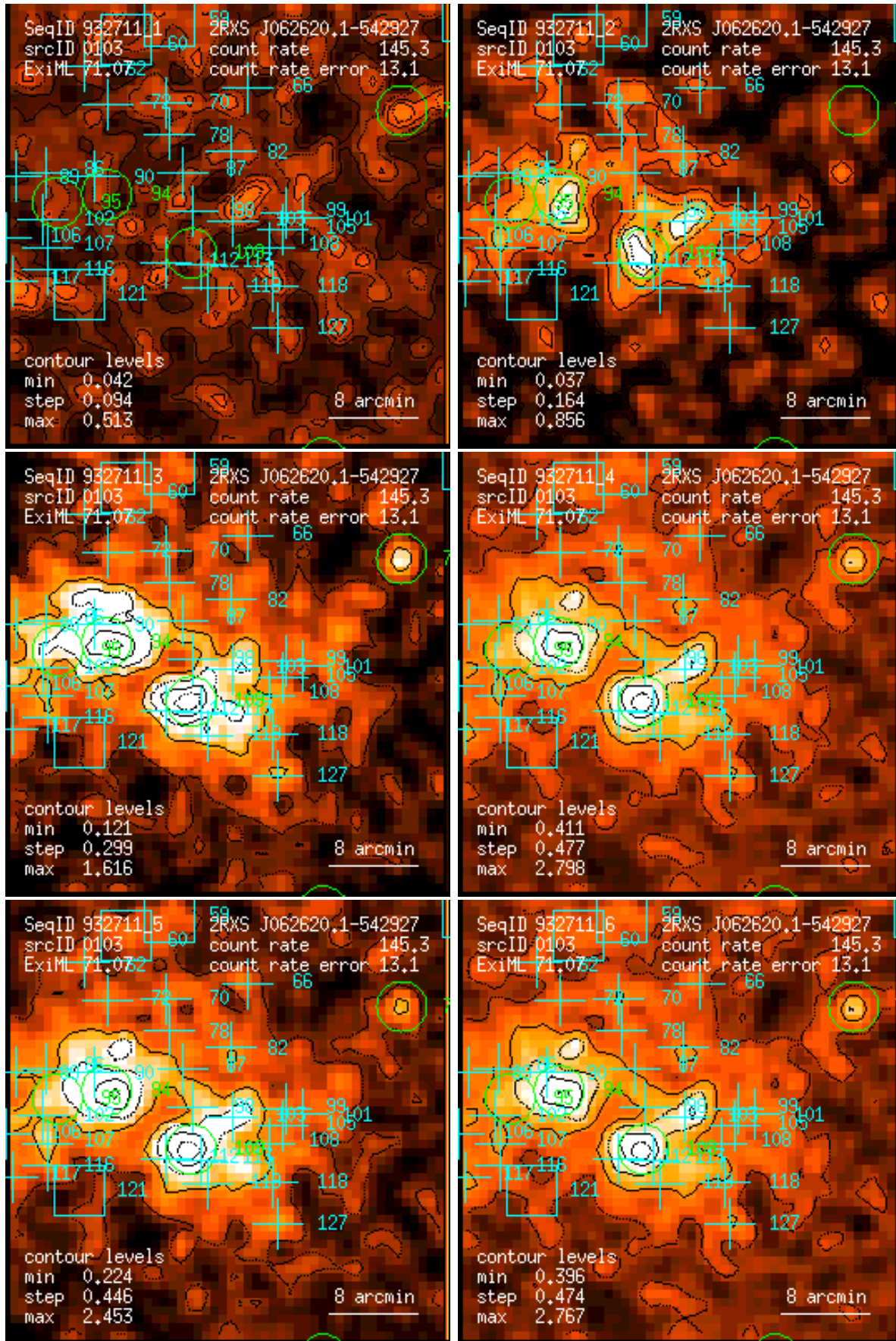
Figure 103: RASS 932711: detection 0103: band rate images, Gaussian filter: (1) PSPC channels 11 – 41, (2) 52 – 90, (3) 91 – 201, (4) 11 – 235, (5) 52 – 201, (6) 11 – 201. Broad band rates in counts/ks. Band rate contour levels in counts/ks/arcmin 2 .
