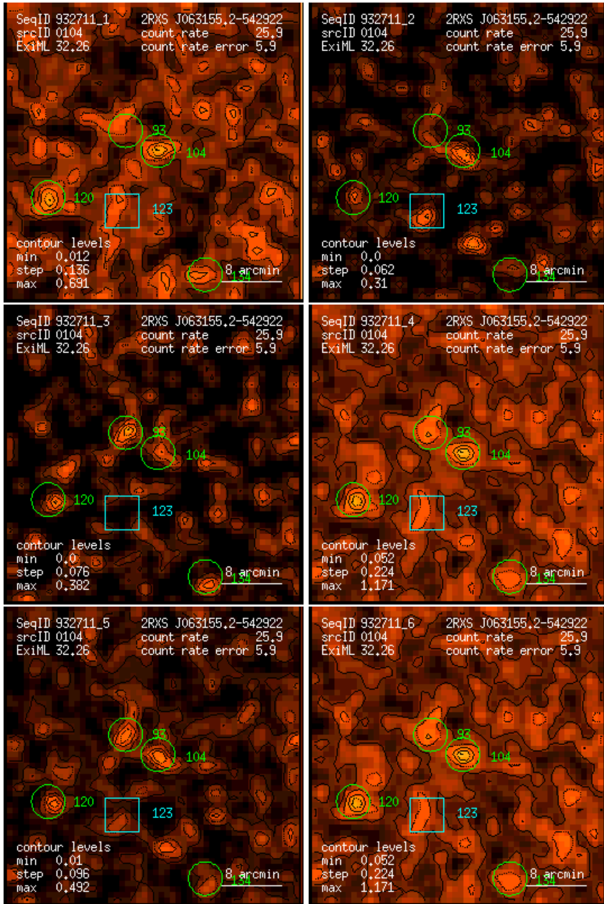
Figure 104: RASS 932711: detection 0104: band rate images, Gaussian filter: (1) PSPC channels 11 – 41, (2) 52 – 90, (3) 91 – 201, (4) 11 – 235, (5) 52 – 201, (6) 11 – 201. Broad band rates in counts/ks. Band rate contour levels in counts/ks/arcmin 2 .
