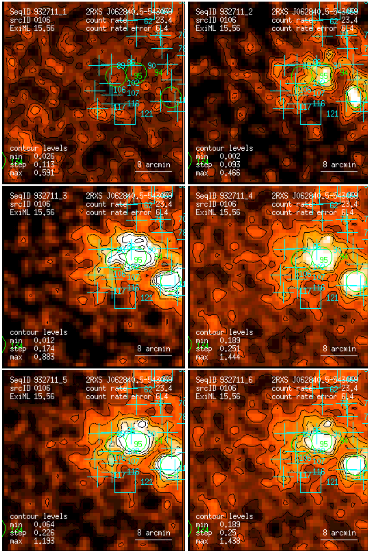
Figure 106: RASS 932711: detection 0106: band rate images, Gaussian filter: (1) PSPC channels 11 – 41, (2) 52 – 90, (3) 91 – 201, (4) 11 – 235, (5) 52 – 201, (6) 11 – 201. Broad band rates in counts/ks. Band rate contour levels in counts/ks/arcmin 2 .
