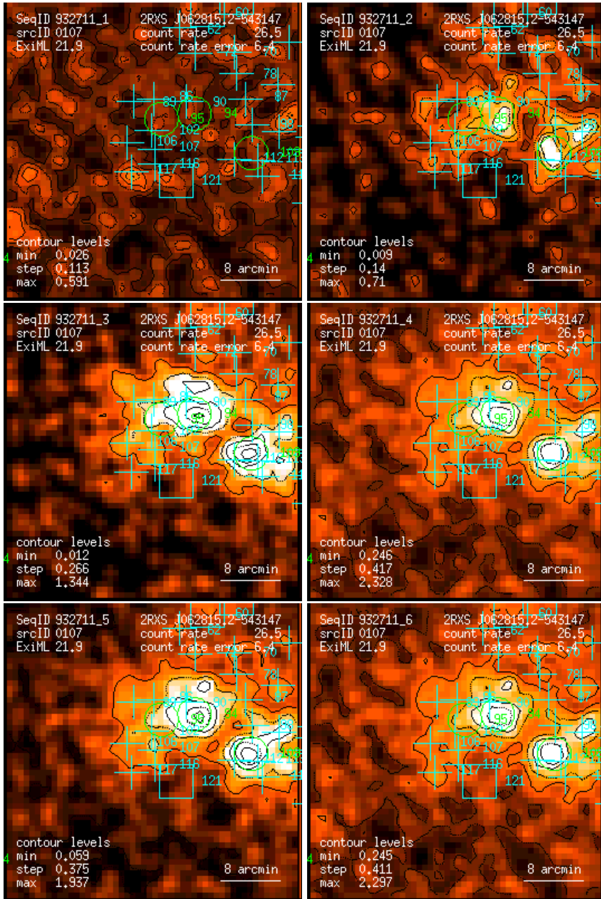
Figure 107: RASS 932711: detection 0107: band rate images, Gaussian filter: (1) PSPC channels 11 – 41, (2) 52 – 90, (3) 91 – 201, (4) 11 – 235, (5) 52 – 201, (6) 11 – 201. Broad band rates in counts/ks. Band rate contour levels in counts/ks/arcmin 2 .
