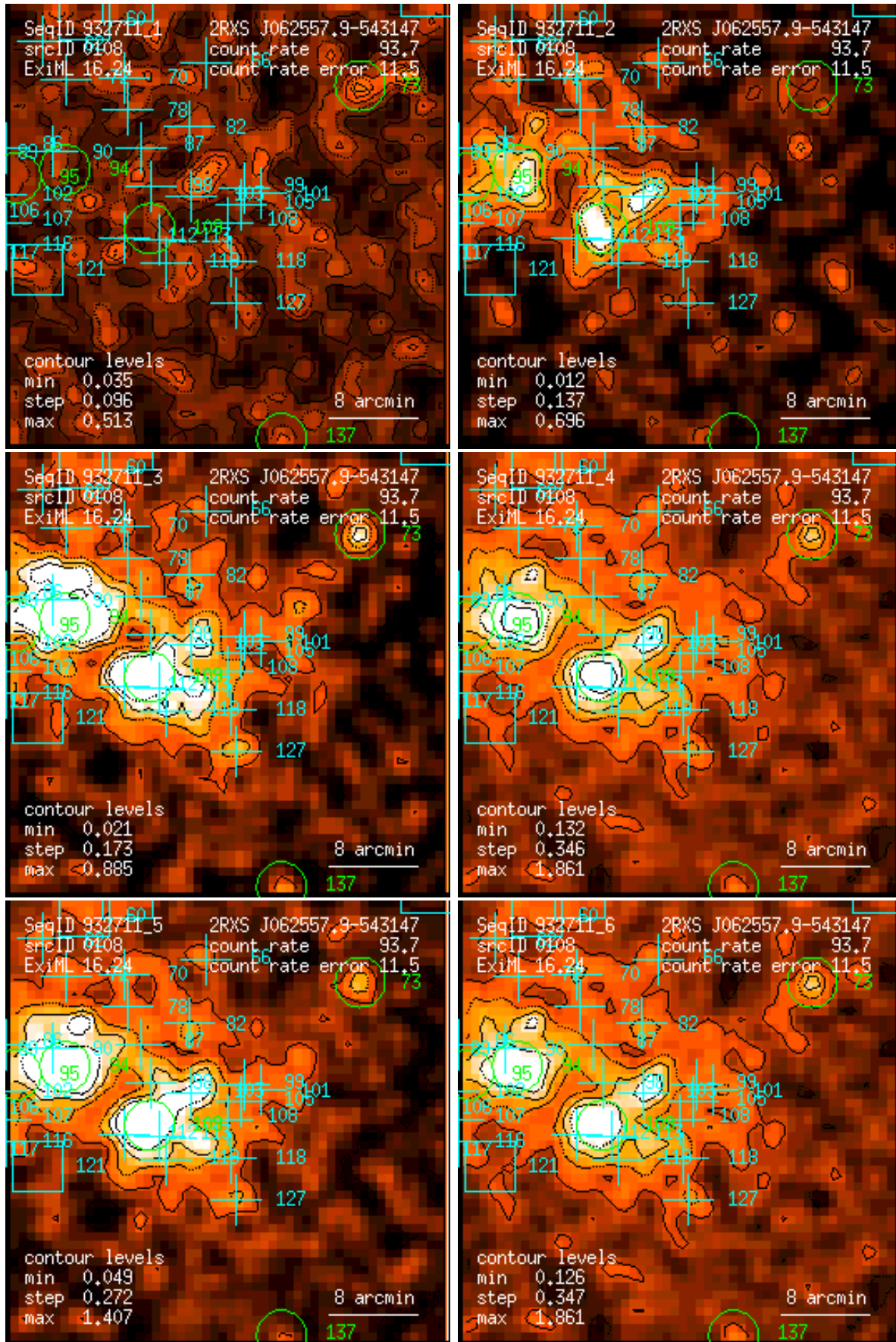
Figure 108: RASS 932711: detection 0108: band rate images, Gaussian filter: (1) PSPC channels 11 – 41, (2) 52 – 90, (3) 91 – 201, (4) 11 – 235, (5) 52 – 201, (6) 11 – 201. Broad band rates in counts/ks. Band rate contour levels in counts/ks/arcmin 2 .
