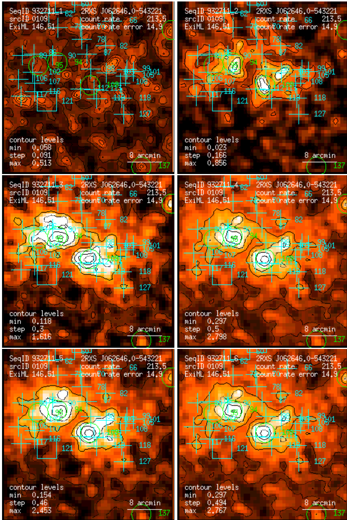
Figure 109: RASS 932711: detection 0109: band rate images, Gaussian filter: (1) PSPC channels 11 – 41, (2) 52 – 90, (3) 91 – 201, (4) 11 – 235, (5) 52 – 201, (6) 11 – 201. Broad band rates in counts/ks. Band rate contour levels in counts/ks/arcmin 2 .
