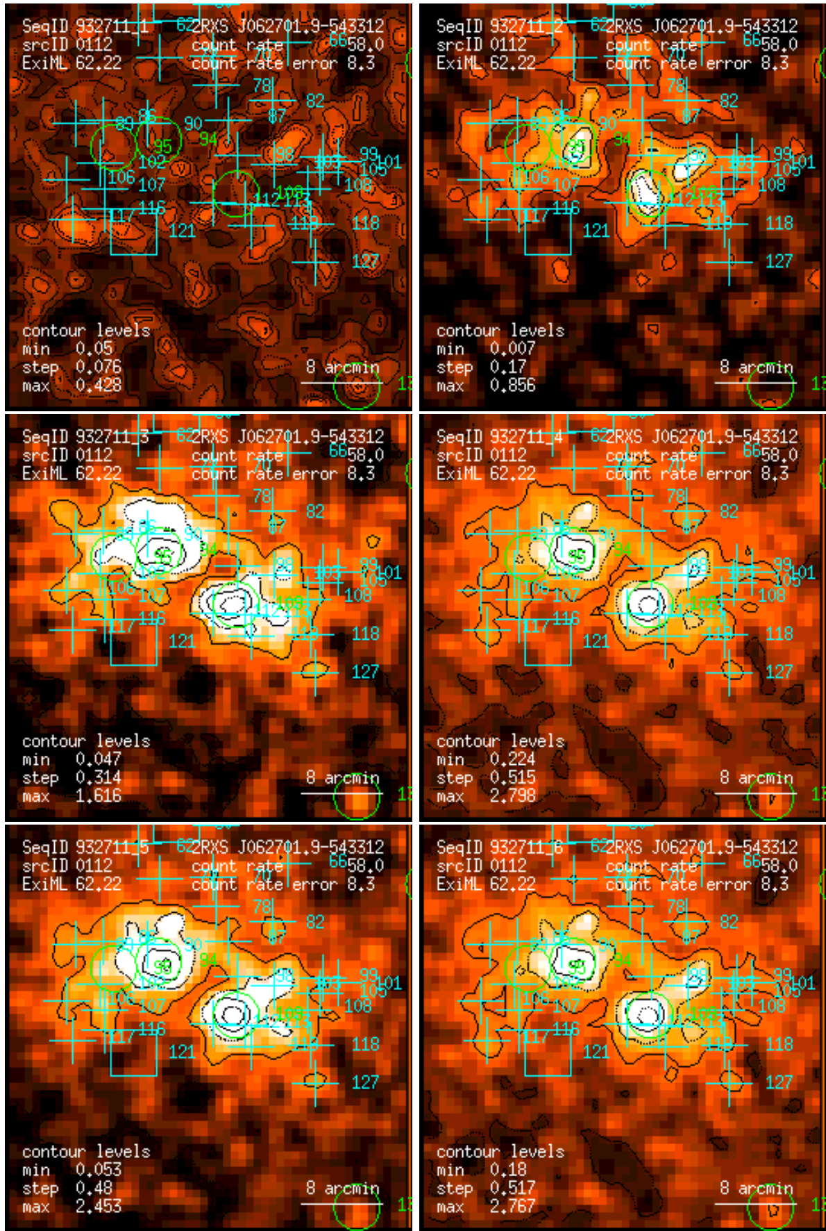
Figure 112: RASS 932711: detection 0112: band rate images, Gaussian filter: (1) PSPC channels 11 – 41, (2) 52 – 90, (3) 91 – 201, (4) 11 – 235, (5) 52 – 201, (6) 11 – 201. Broad band rates in counts/ks. Band rate contour levels in counts/ks/arcmin 2 .
