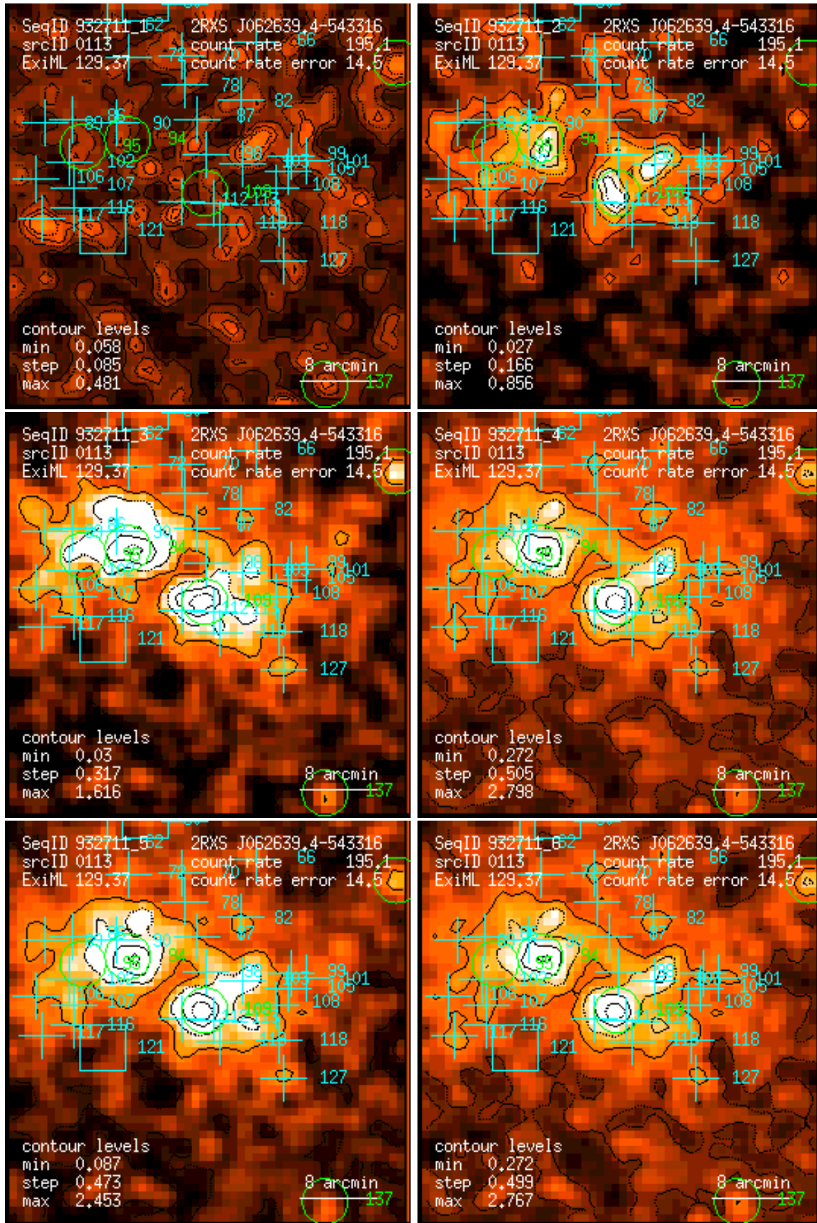
Figure 113: RASS 932711: detection 0113: band rate images, Gaussian filter: (1) PSPC channels 11 – 41, (2) 52 – 90, (3) 91 – 201, (4) 11 – 235, (5) 52 – 201, (6) 11 – 201. Broad band rates in counts/ks. Band rate contour levels in counts/ks/arcmin 2 .
