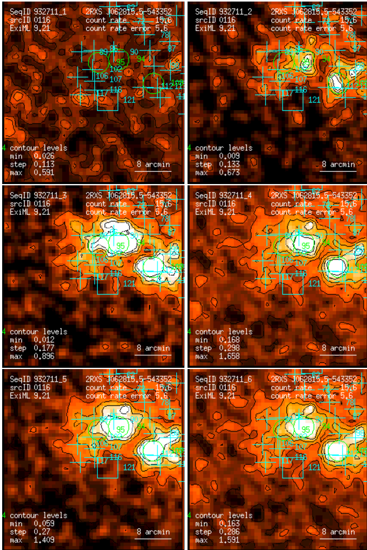
Figure 116: RASS 932711: detection 0116: band rate images, Gaussian filter: (1) PSPC channels 11 – 41, (2) 52 – 90, (3) 91 – 201, (4) 11 – 235, (5) 52 – 201, (6) 11 – 201. Broad band rates in counts/ks. Band rate contour levels in counts/ks/arcmin 2 .
