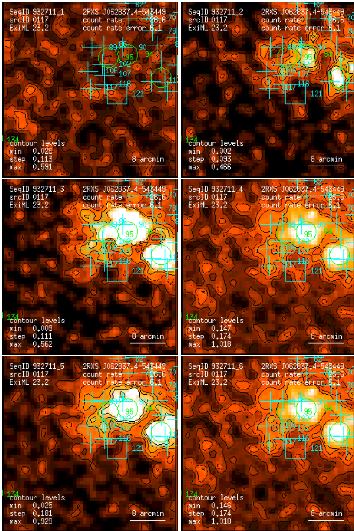
Figure 117: RASS 932711: detection 0117: band rate images, Gaussian filter: (1) PSPC channels 11 – 41, (2) 52 – 90, (3) 91 – 201, (4) 11 – 235, (5) 52 – 201, (6) 11 – 201. Broad band rates in counts/ks. Band rate contour levels in counts/ks/arcmin 2 .
