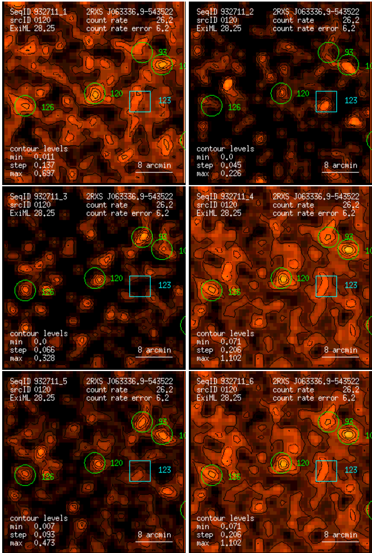
Figure 120: RASS 932711: detection 0120: band rate images, Gaussian filter: (1) PSPC channels 11 – 41, (2) 52 – 90, (3) 91 – 201, (4) 11 – 235, (5) 52 – 201, (6) 11 – 201. Broad band rates in counts/ks. Band rate contour levels in counts/ks/arcmin 2 .
