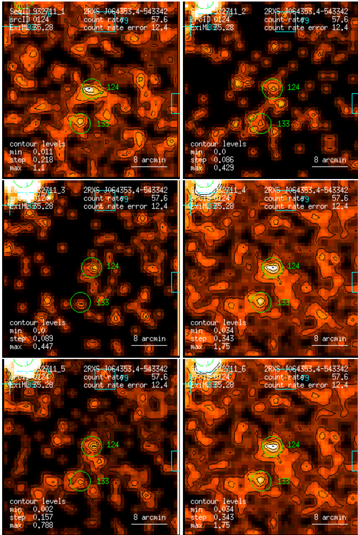
Figure 124: RASS 932711: detection 0124: band rate images, Gaussian filter: (1) PSPC channels 11 – 41, (2) 52 – 90, (3) 91 – 201, (4) 11 – 235, (5) 52 – 201, (6) 11 – 201. Broad band rates in counts/ks. Band rate contour levels in counts/ks/arcmin 2 .
