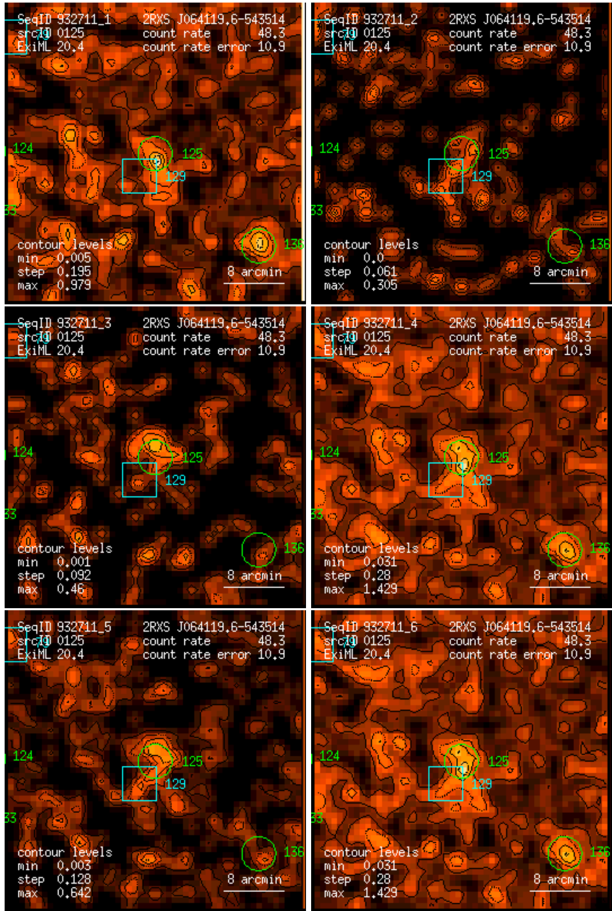
Figure 125: RASS 932711: detection 0125: band rate images, Gaussian filter: (1) PSPC channels 11 – 41, (2) 52 – 90, (3) 91 – 201, (4) 11 – 235, (5) 52 – 201, (6) 11 – 201. Broad band rates in counts/ks. Band rate contour levels in counts/ks/arcmin 2 .
