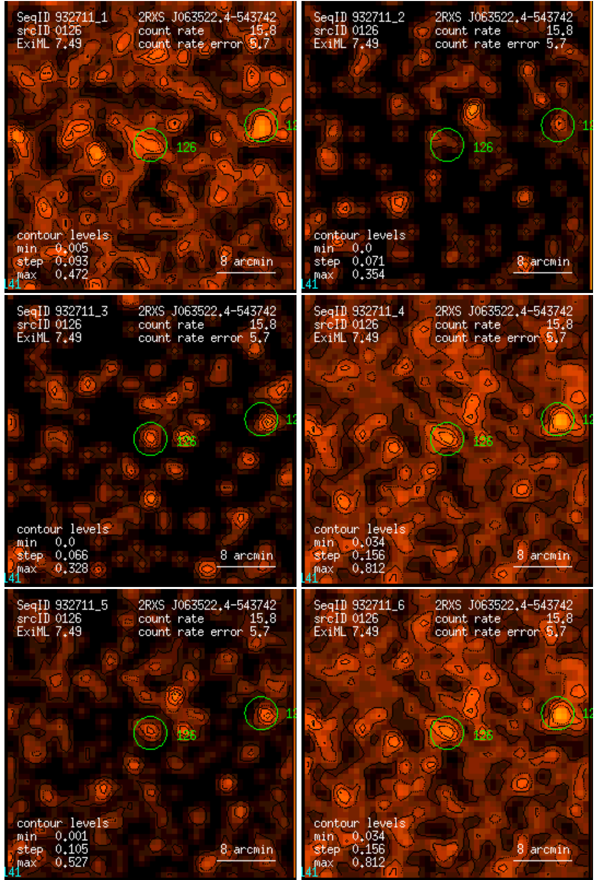
Figure 126: RASS 932711: detection 0126: band rate images, Gaussian filter: (1) PSPC channels 11 – 41, (2) 52 – 90, (3) 91 – 201, (4) 11 – 235, (5) 52 – 201, (6) 11 – 201. Broad band rates in counts/ks. Band rate contour levels in counts/ks/arcmin 2 .
