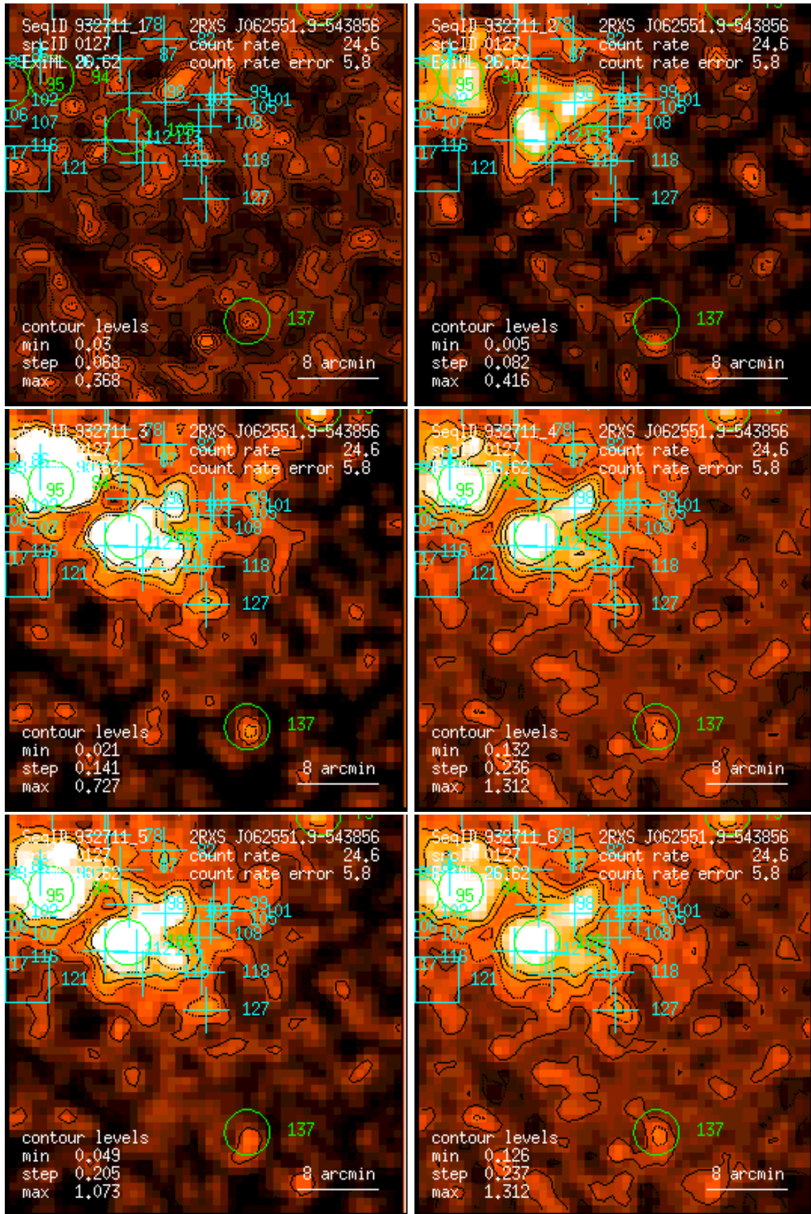
Figure 127: RASS 932711: detection 0127: band rate images, Gaussian filter: (1) PSPC channels 11 – 41, (2) 52 – 90, (3) 91 – 201, (4) 11 – 235, (5) 52 – 201, (6) 11 – 201. Broad band rates in counts/ks. Band rate contour levels in counts/ks/arcmin 2 .
