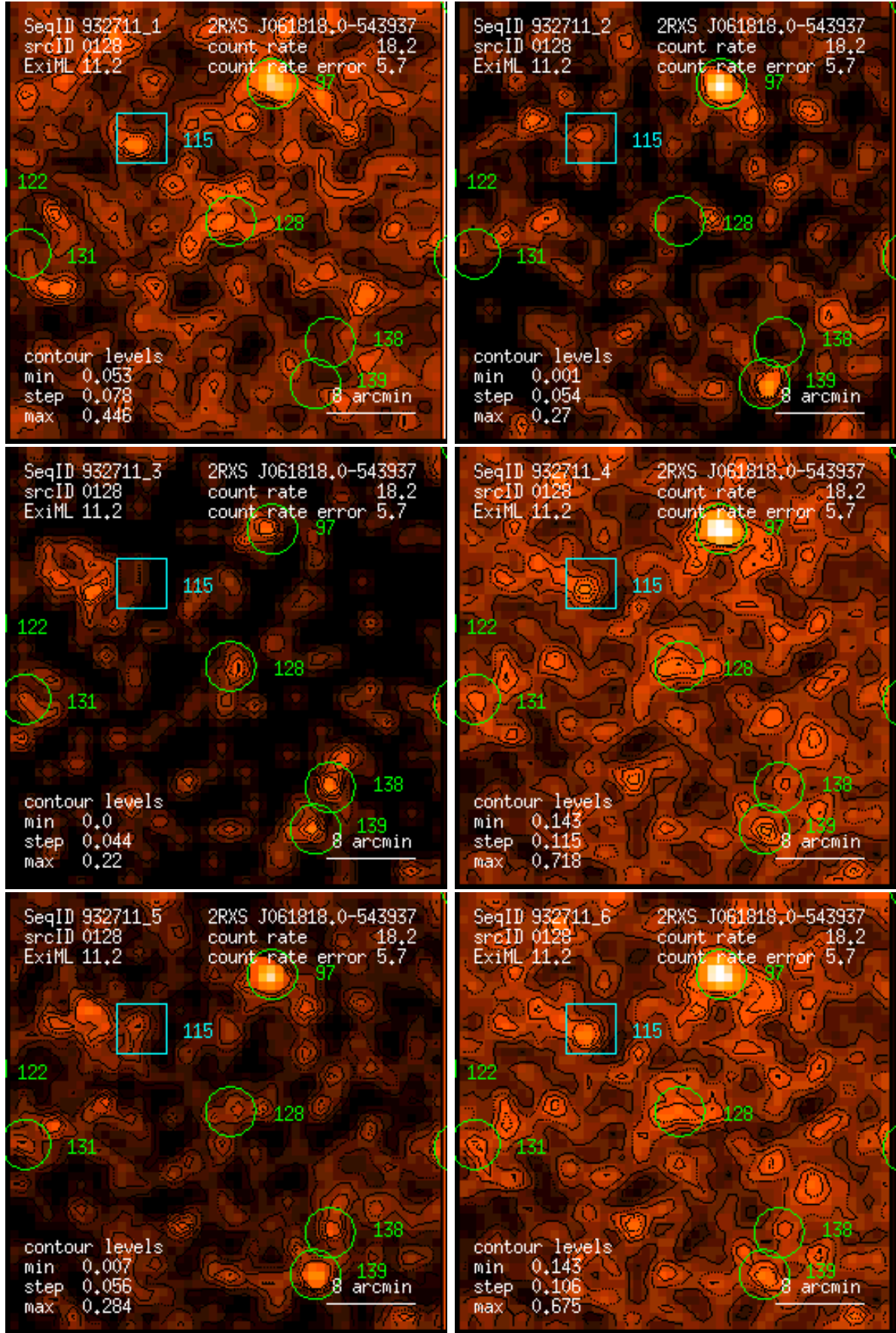
Figure 128: RASS 932711: detection 0128: band rate images, Gaussian filter: (1) PSPC channels 11 – 41, (2) 52 – 90, (3) 91 – 201, (4) 11 – 235, (5) 52 – 201, (6) 11 – 201. Broad band rates in counts/ks. Band rate contour levels in counts/ks/arcmin 2 .
