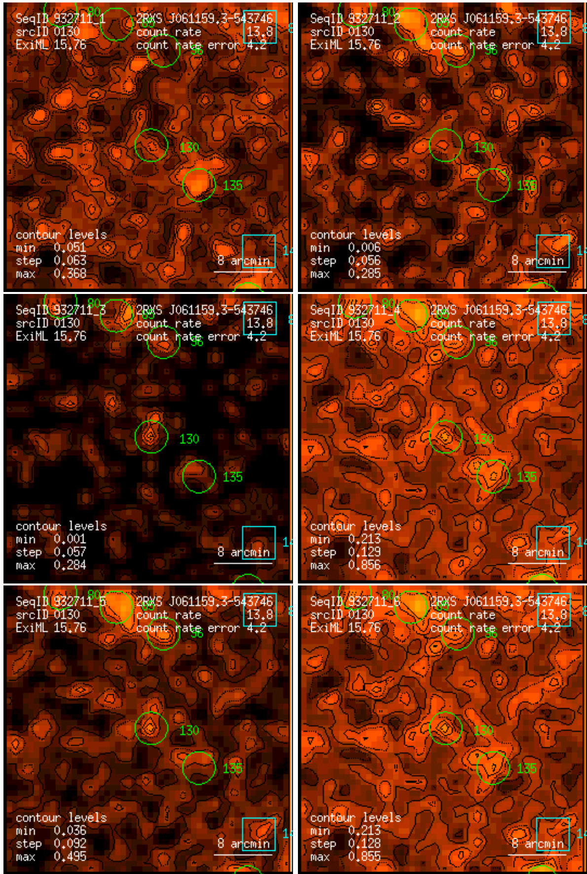
Figure 130: RASS 932711: detection 0130: band rate images, Gaussian filter: (1) PSPC channels 11 – 41, (2) 52 – 90, (3) 91 – 201, (4) 11 – 235, (5) 52 – 201, (6) 11 – 201. Broad band rates in counts/ks. Band rate contour levels in counts/ks/arcmin 2 .
