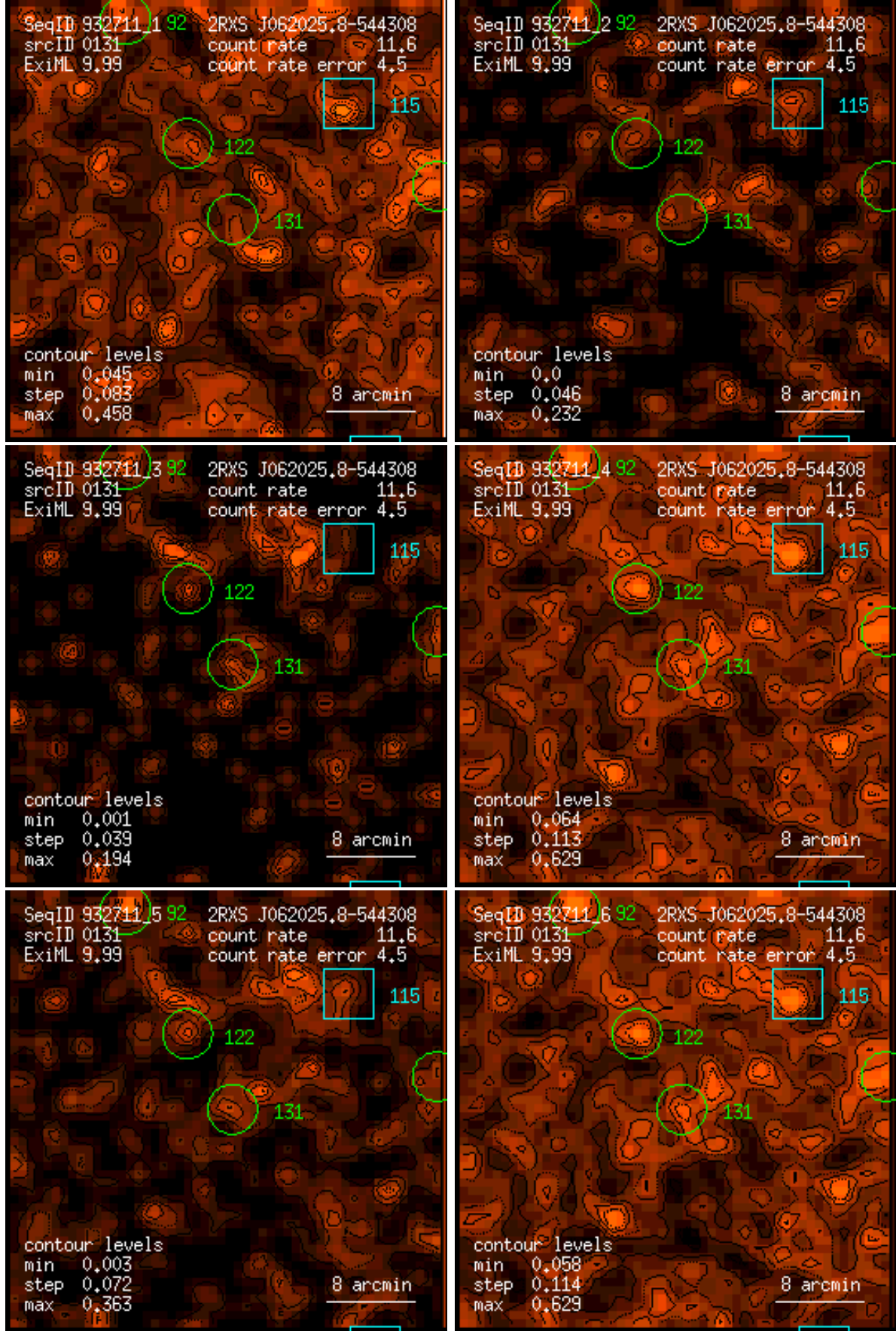
Figure 131: RASS 932711: detection 0131: band rate images, Gaussian filter: (1) PSPC channels 11 – 41, (2) 52 – 90, (3) 91 – 201, (4) 11 – 235, (5) 52 – 201, (6) 11 – 201. Broad band rates in counts/ks. Band rate contour levels in counts/ks/arcmin 2 .
