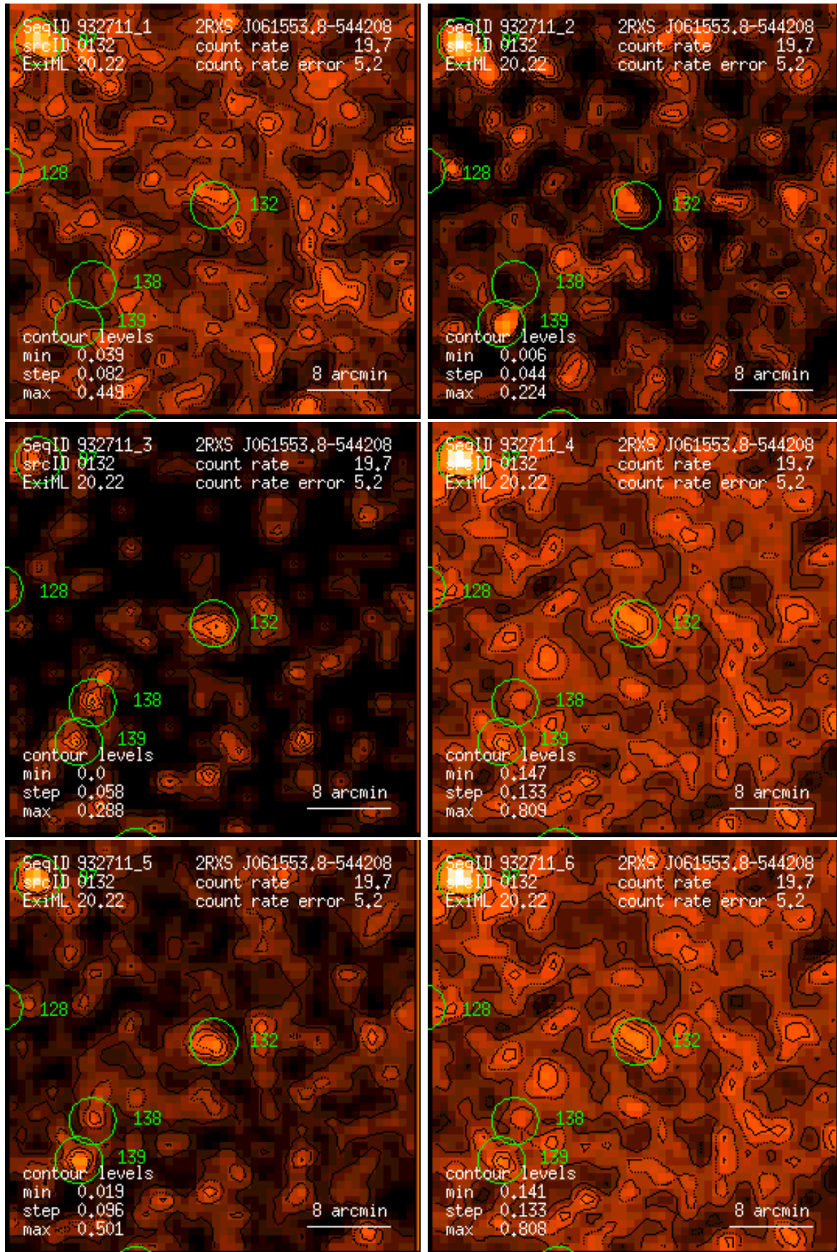
Figure 132: RASS 932711: detection 0132: band rate images, Gaussian filter: (1) PSPC channels 11 – 41, (2) 52 – 90, (3) 91 – 201, (4) 11 – 235, (5) 52 – 201, (6) 11 – 201. Broad band rates in counts/ks. Band rate contour levels in counts/ks/arcmin 2 .
